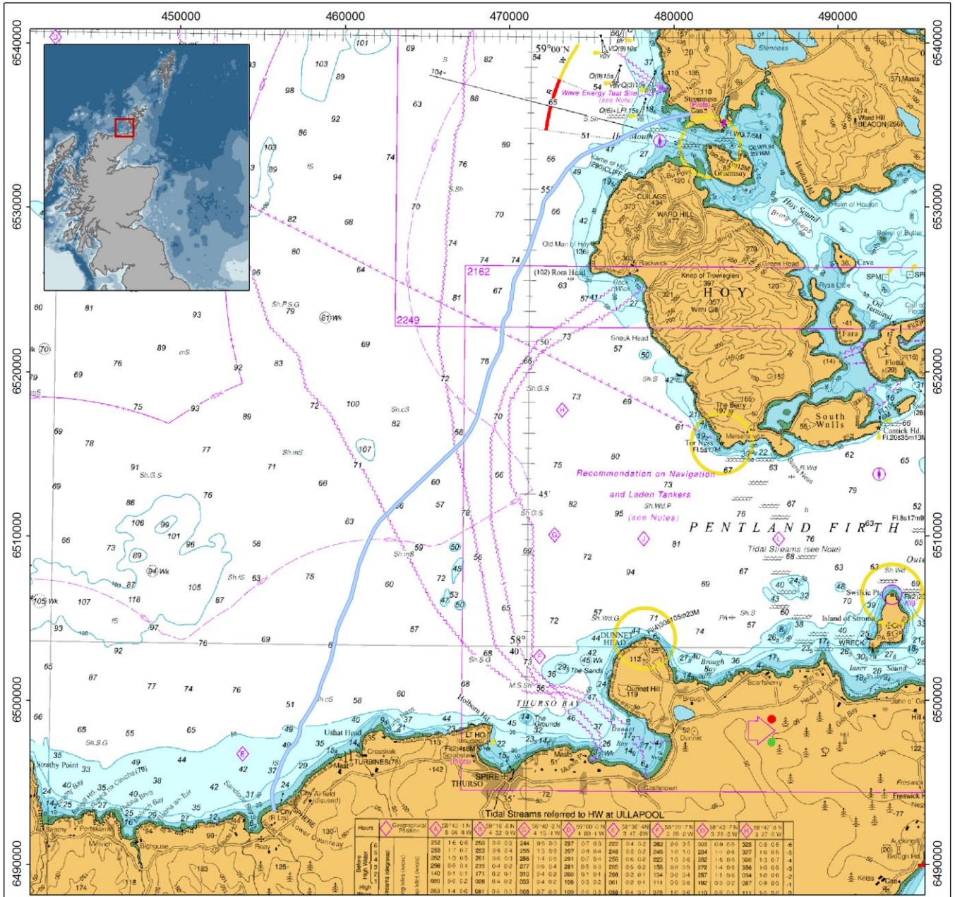
Figure 1: Proposed cable installation corridor
