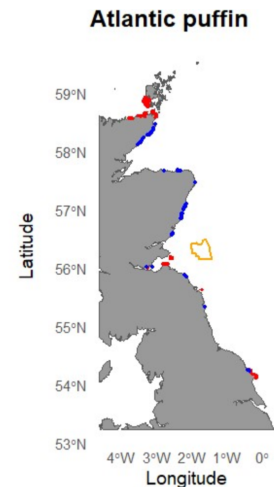
Figure A.5: Sites Included in the Breeding Season Apportioning Calculations for Atlantic Puffin. The Orange Area Is the Site of the Proposed Development. The Red Areas Represent the SPAs and the Blue Areas Represent the Non-Designated Sites Included in the Apportioning Calculations.
