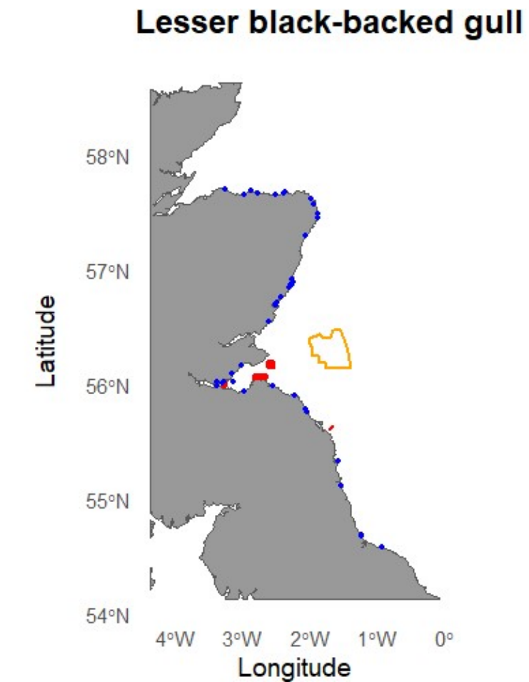
Figure A.4: Sites Included in the Breeding Season Apportioning Calculations for Lesser Black-Backed Gull. The Orange Area Is the Site of the Proposed Development. The Red Areas Represent the SPAs and the Blue Areas Represent the Non-Designated Sites Included in the Apportioning Calculations.
