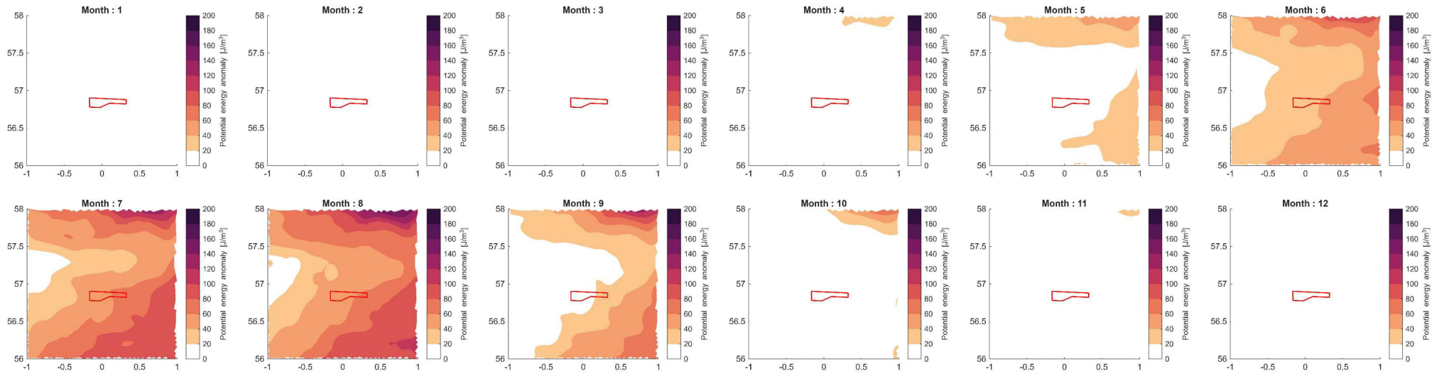
Plate 3.14: Monthly Averaged Potential Energy Anomaly Maps
