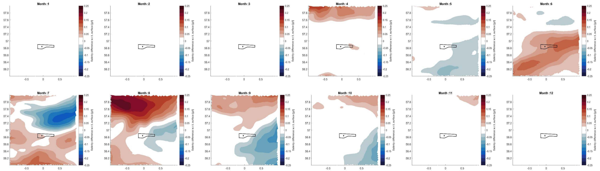
Plate 3.11: Salinity Difference Between Surface and Seabed (Negative Values Mean Higher Concentration at Seabed than Surface and Positive Values Vice Versa)
