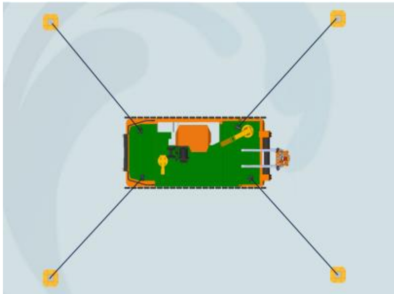
Figure 14. Multicat temporary 4 point mooring for drilling operation
