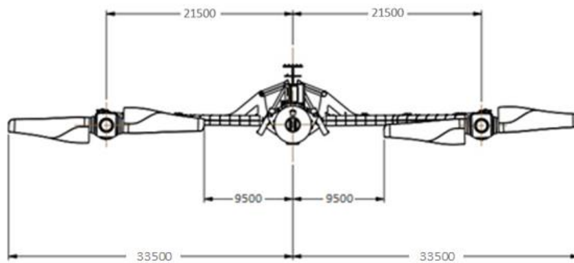
Figure 1 Orbital O2.4 in transport mode
