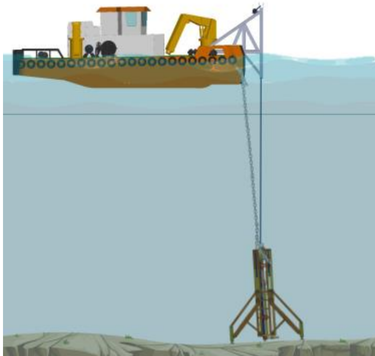
Figure 15. Drilling rig lowered to seabed
