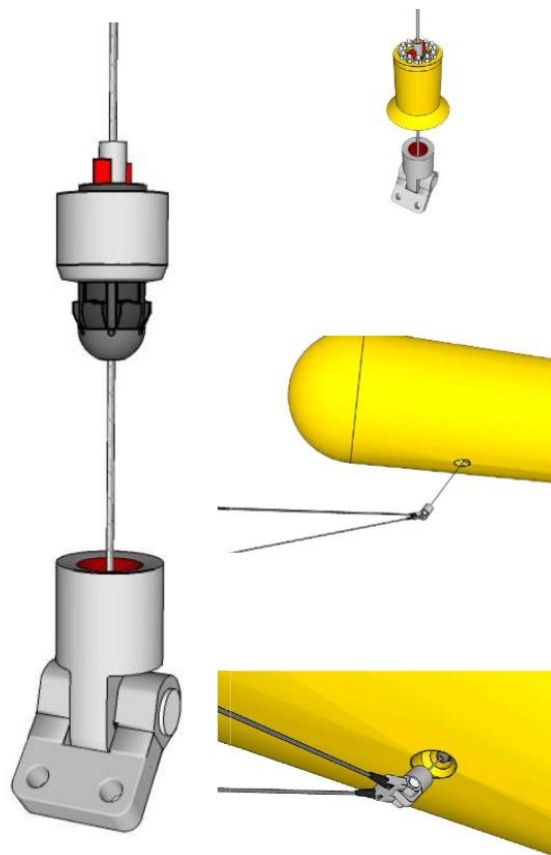
Figure 12 Orbital O2.4 mooring connector
