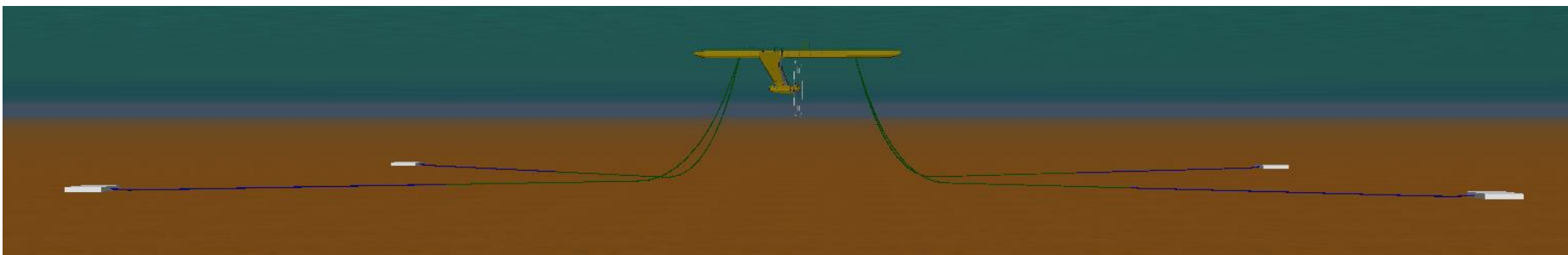
Figure 5 Orbital O2.4 mooring system at slack tide (green lines are 95mm Studlink chain, blue lines are 115mm studlink)
