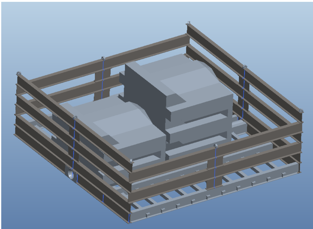
Figure 8 Anchor basket with ballast
