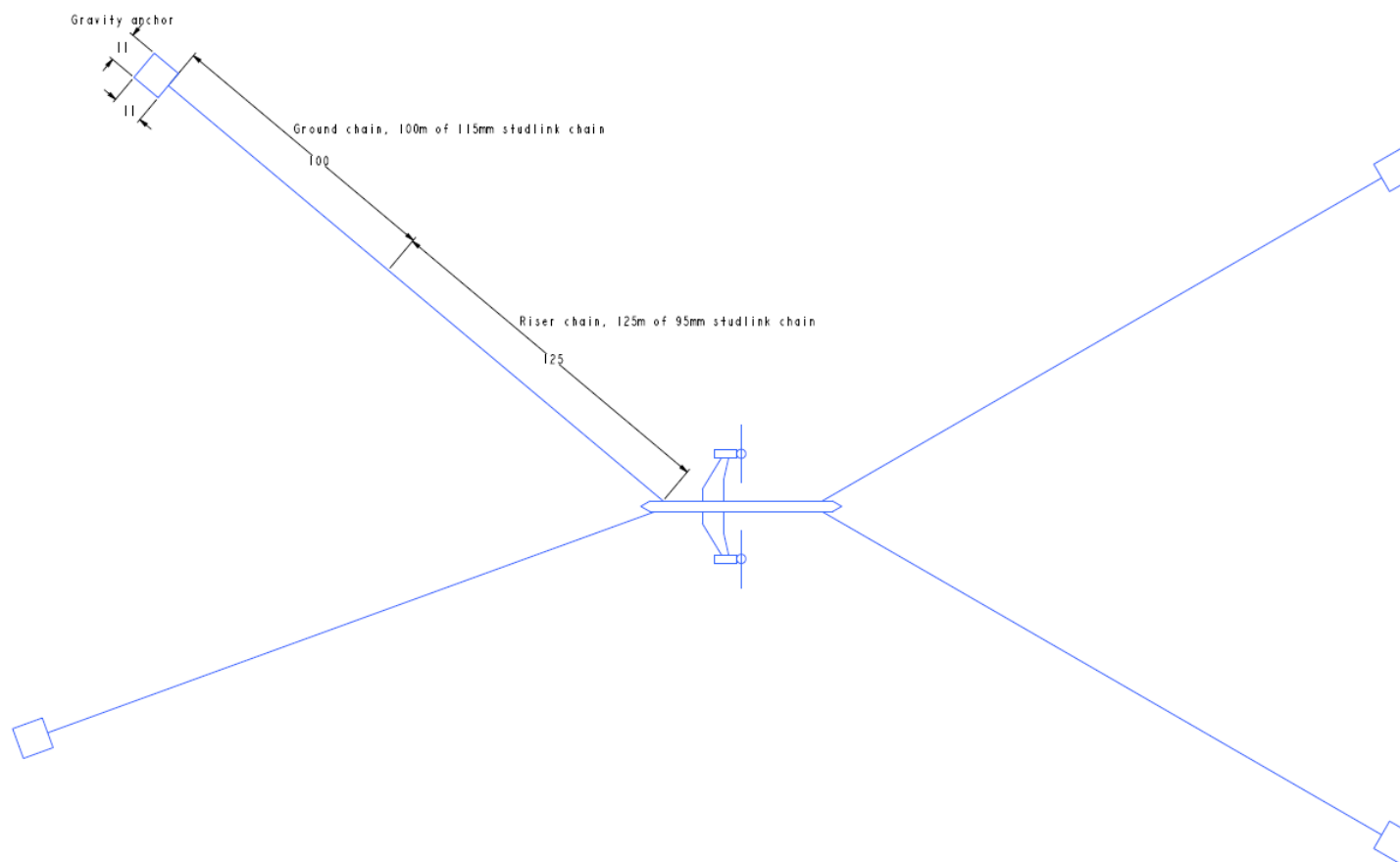
Figure 7 Schematic showing make up of each mooring line
