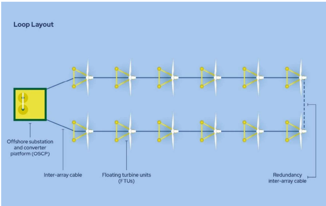
Figure 5-15 Loop layout option
