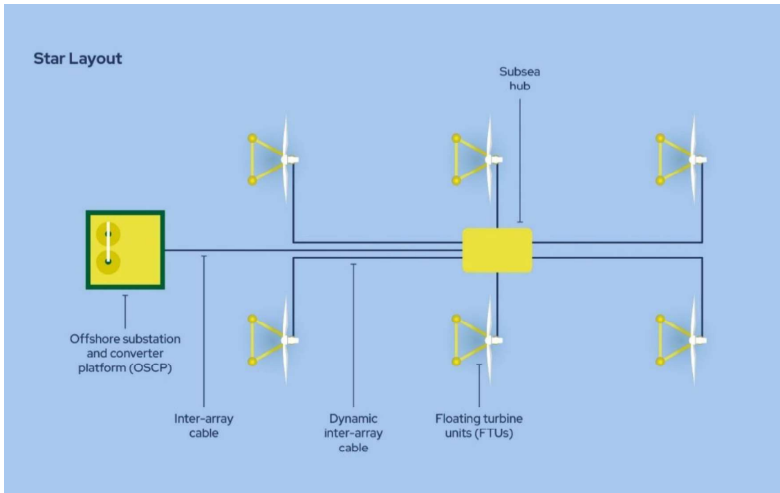
Figure 5-17 Star layout option
