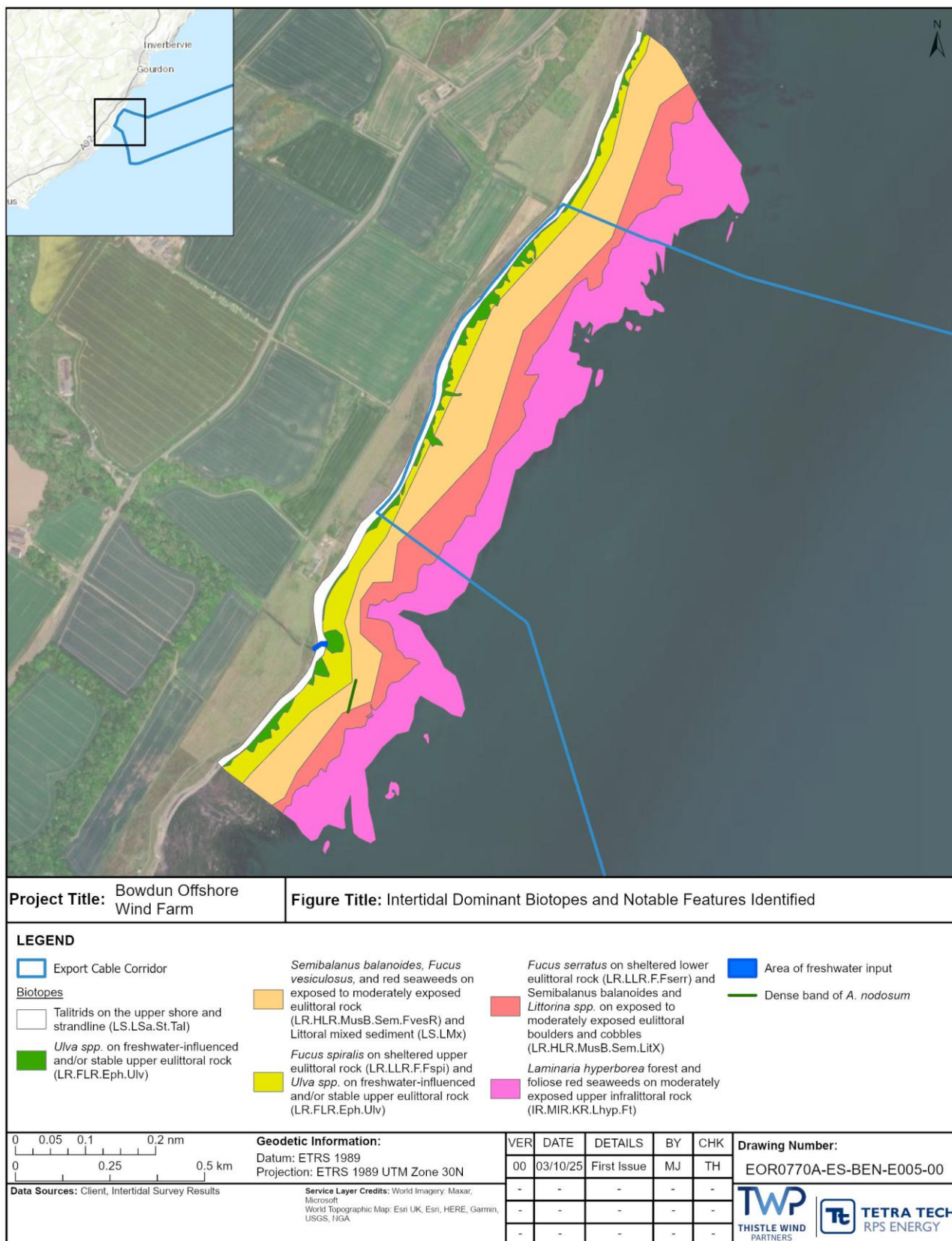
Figure 8.6: Intertidal Dominant Biotopes and Notable Features Identified
