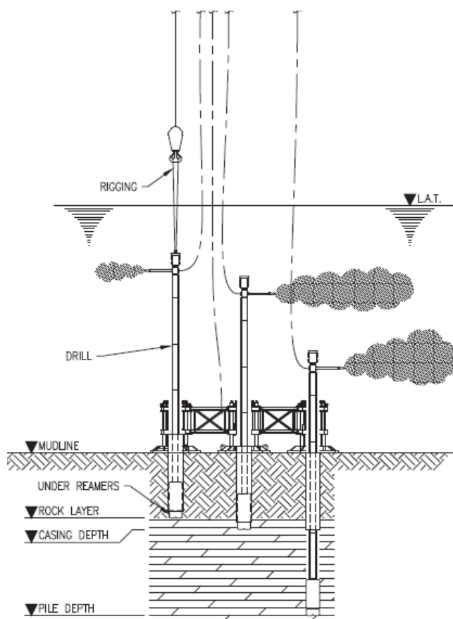
Figure 6-4: Illustration of drilling operations
