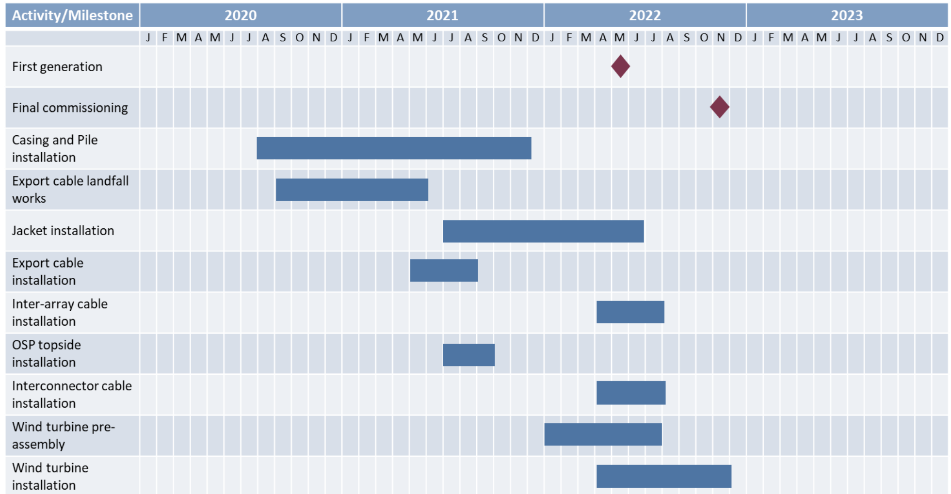
Figure 4-1: Construction Programme
