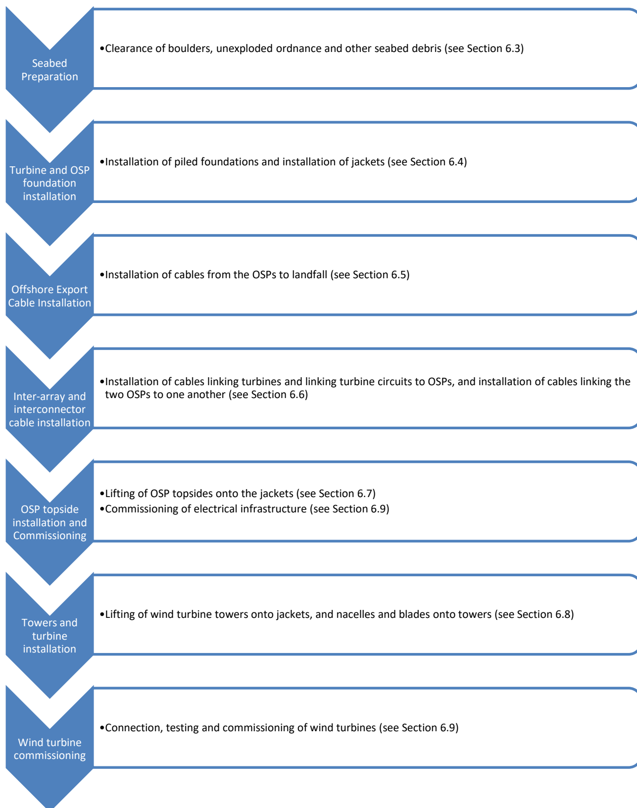
Figure 6-1: Overview of the Wind Farm and O&TW installation process
