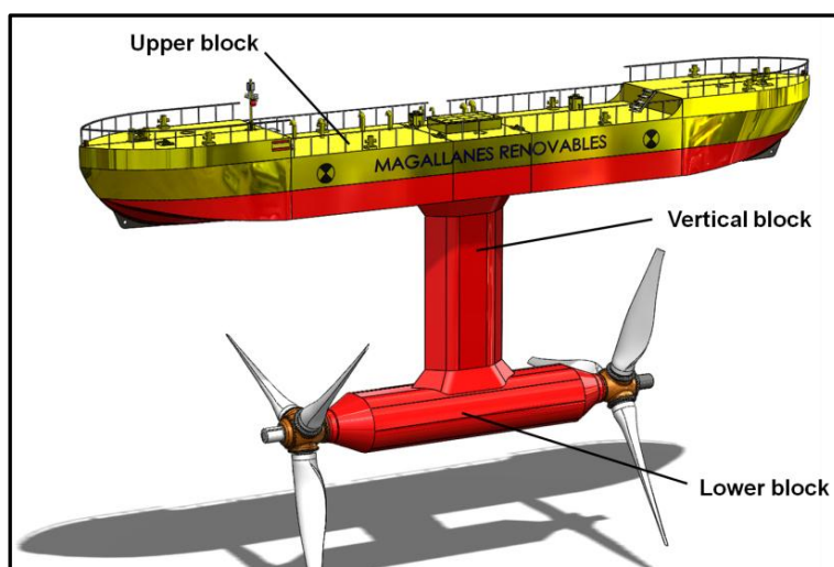
Figure 3. Device layout
