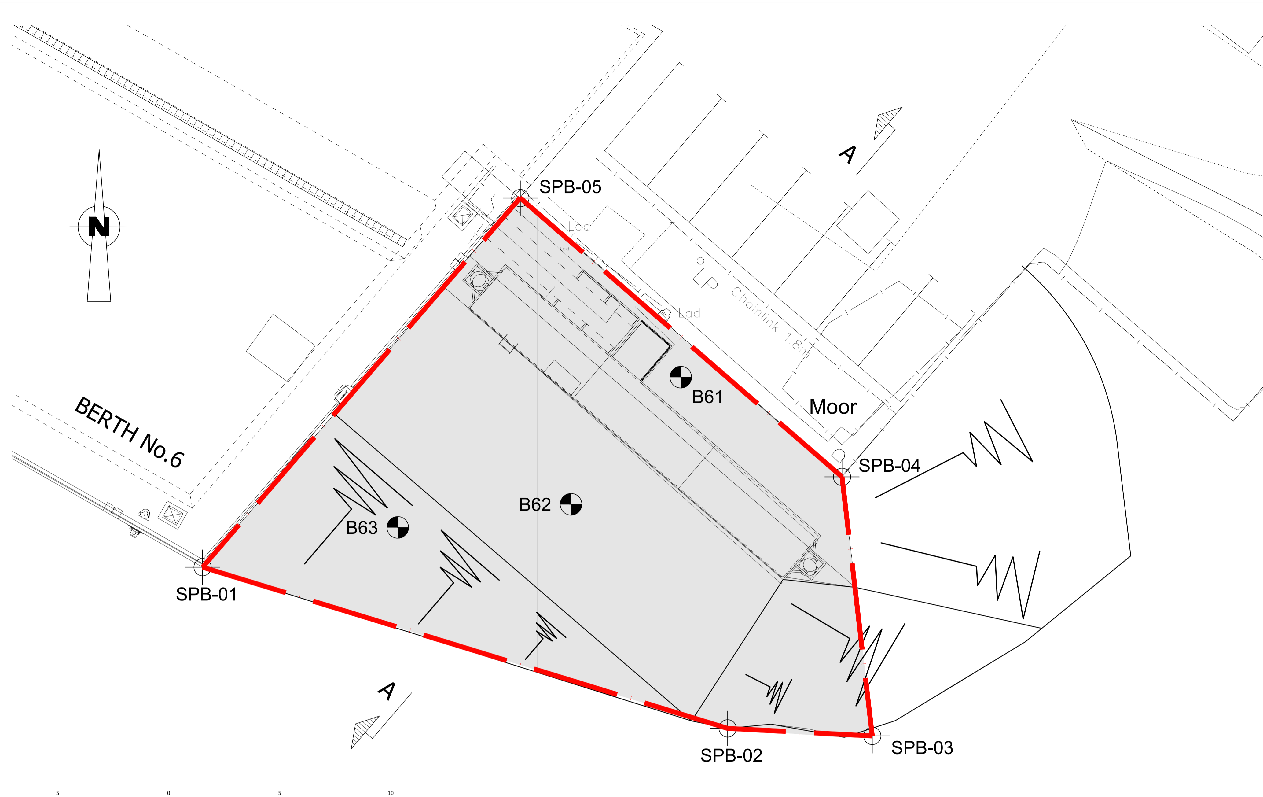
BERTH No.6 - EAST SIDE - SAMPLING PLAN (scale 1:100)
