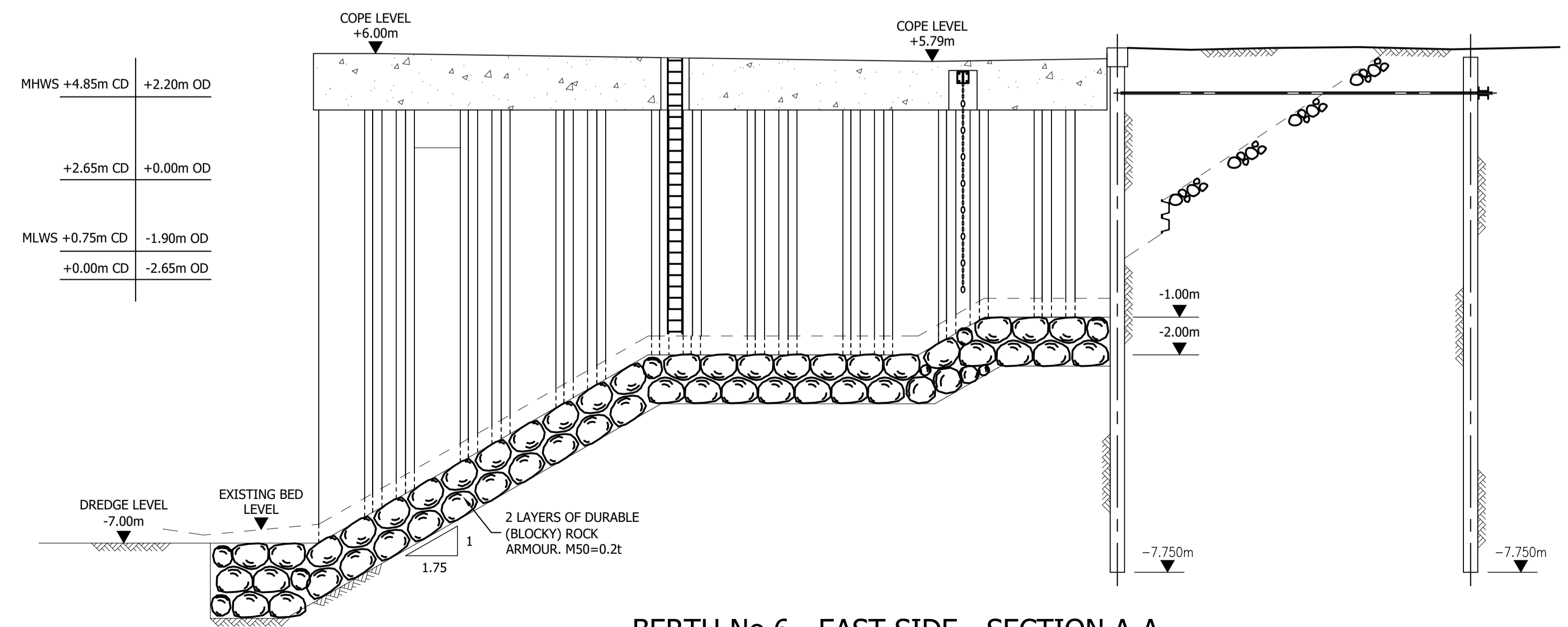
BERTH No.6 - EAST SIDE - SECTION A-A (scale 1:100)
