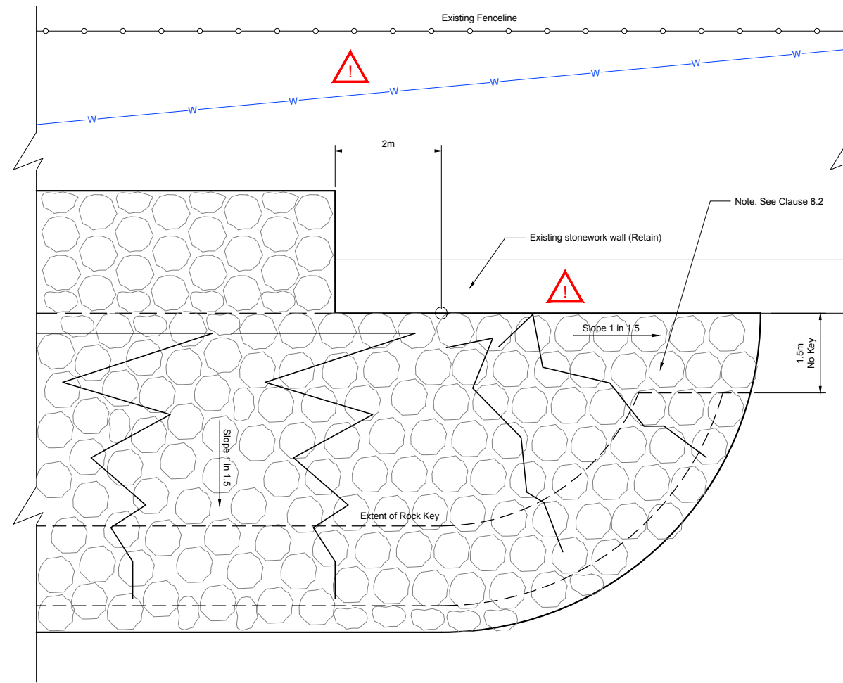
East Tie-in Detail 1:50
