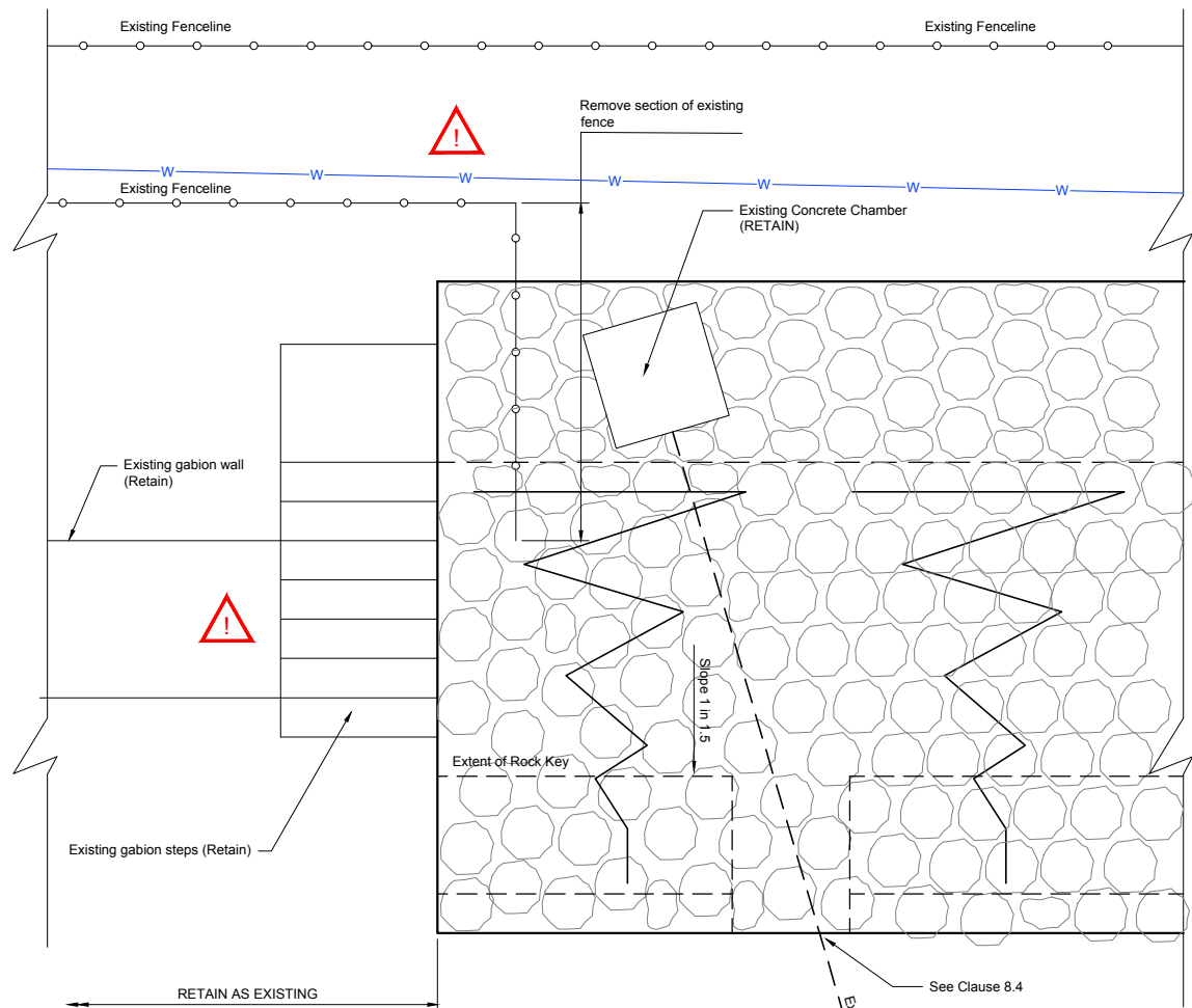
West Tie-in Detail 1:50
