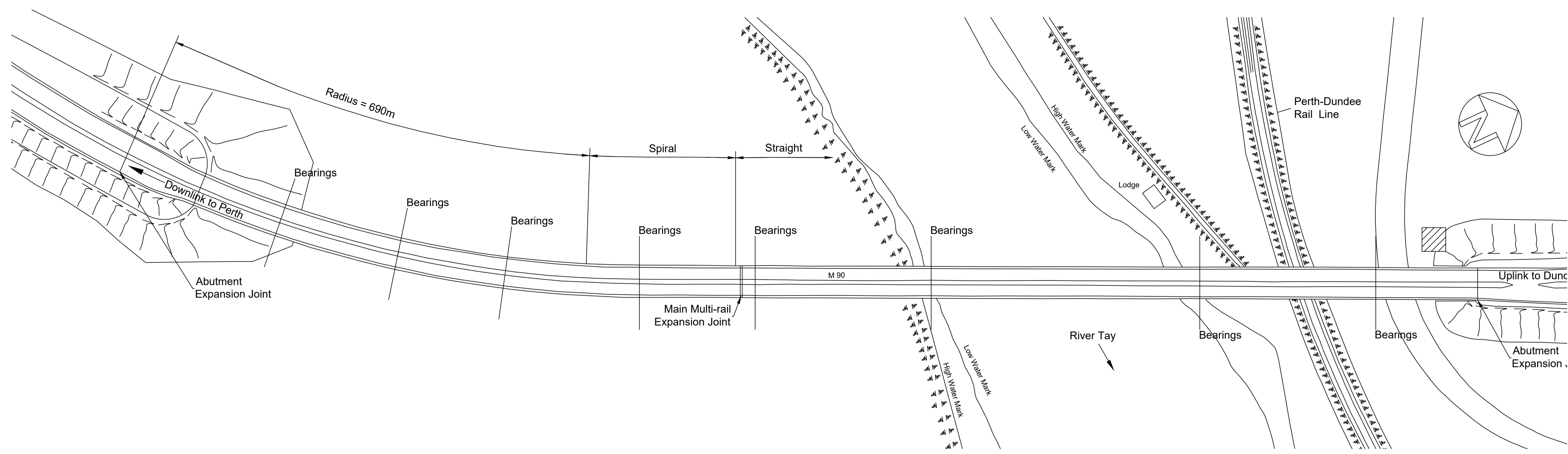
Plan of Bridge Scale 1:1500
