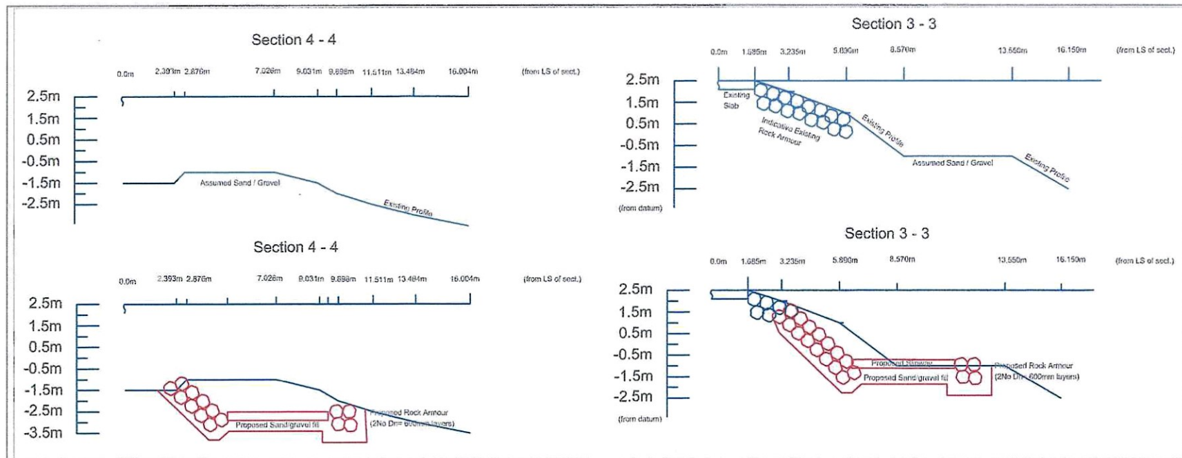
Proposed Sections 4 & 3
