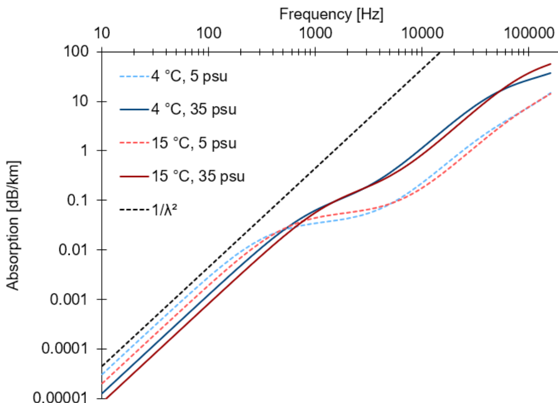
Figure 8-12: Absorption loss coefficient (dB/km) for various salinities and temperature.
