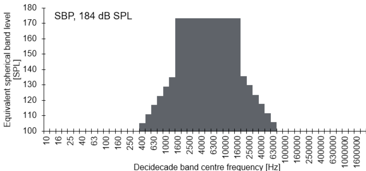
Figure 4-7. Chirper/Pinger type SBP band levels.
