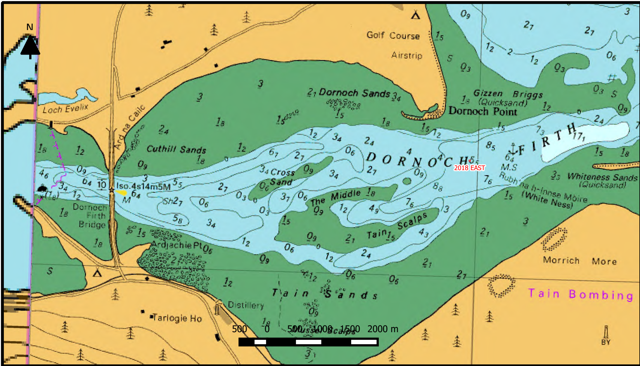
FIGURE 2 - LOCATION PLAN USING ADMIRALTY CHART BASE SHOWING DORNOCH FIRTH. SITE AREAS FOR PROPOSED EAST SITE OUTLINED IN RED
