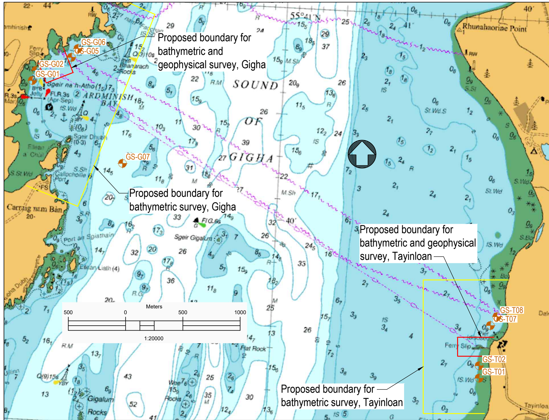
Proposed Ground Investigation and Geophysical Works Layout, outside terminal areas [1:20,000]
