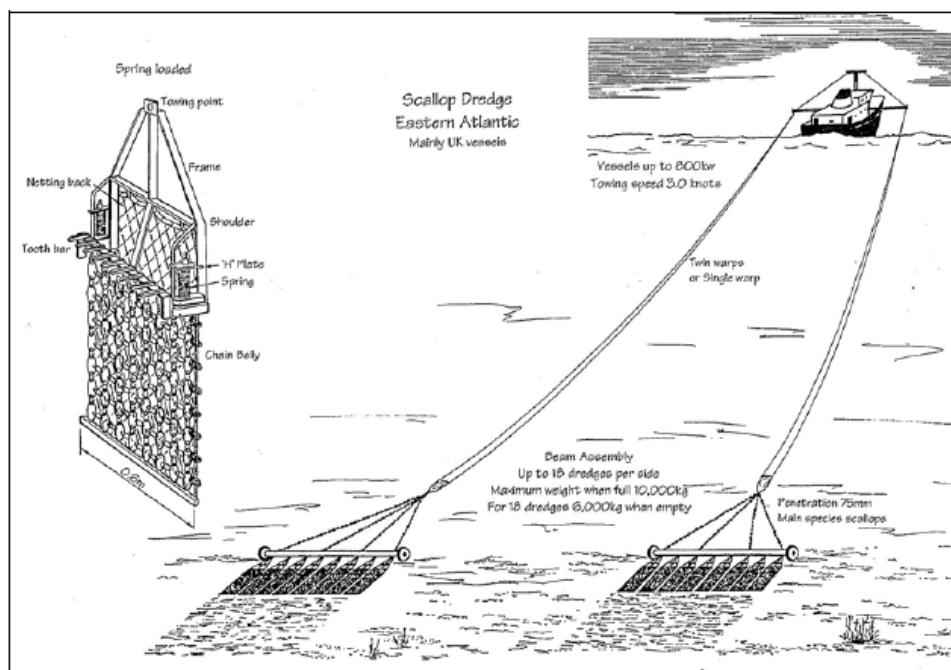
Figure 8.4 Plan View of Scallop Dredger (Ref. iii)
