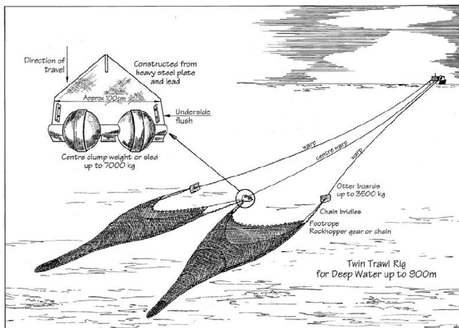
Figure 8.2 Twin Demersal Otter Trawl (Ref. iii)
