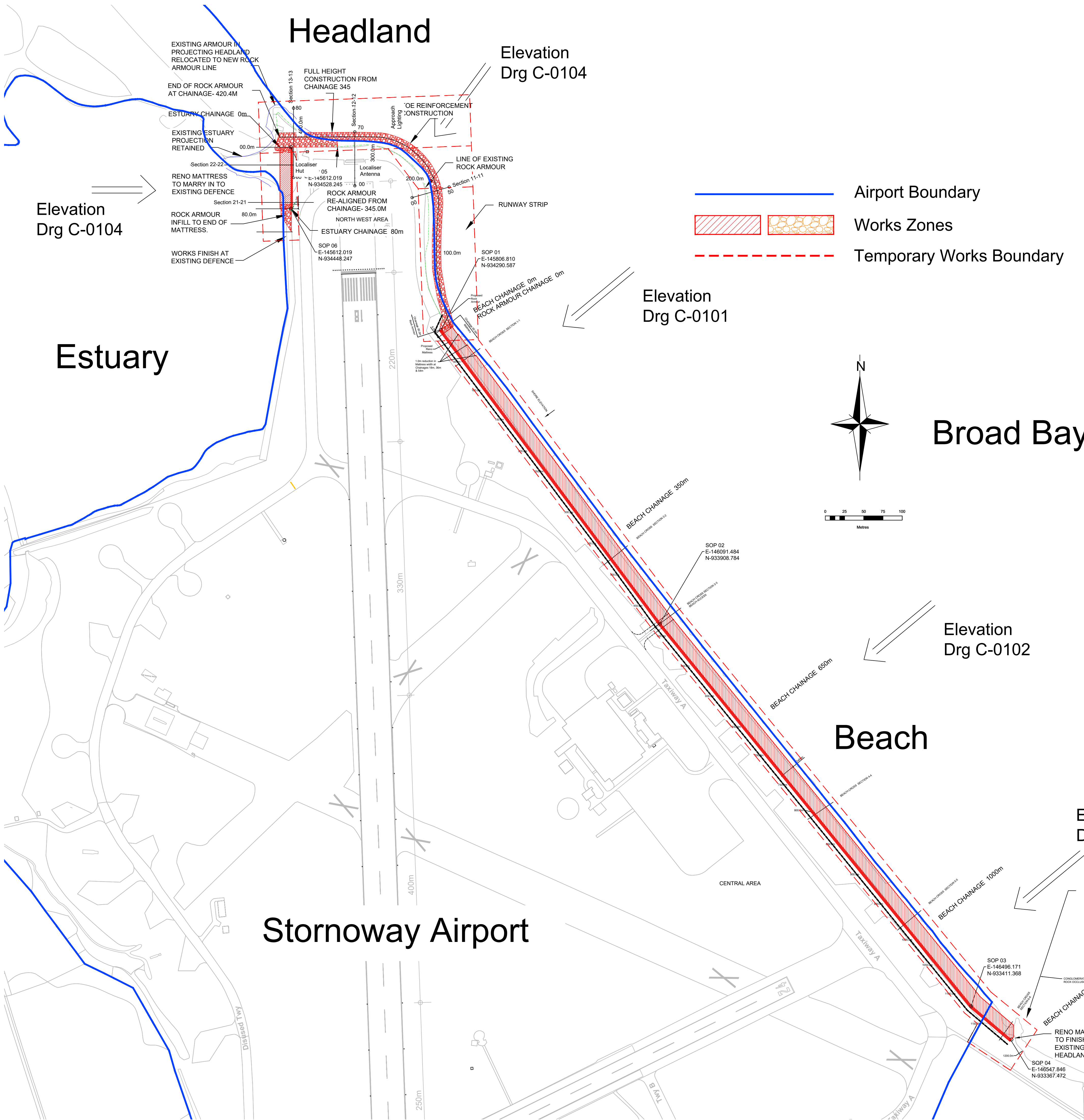
Overall Airport Plan Scale 1:10000
