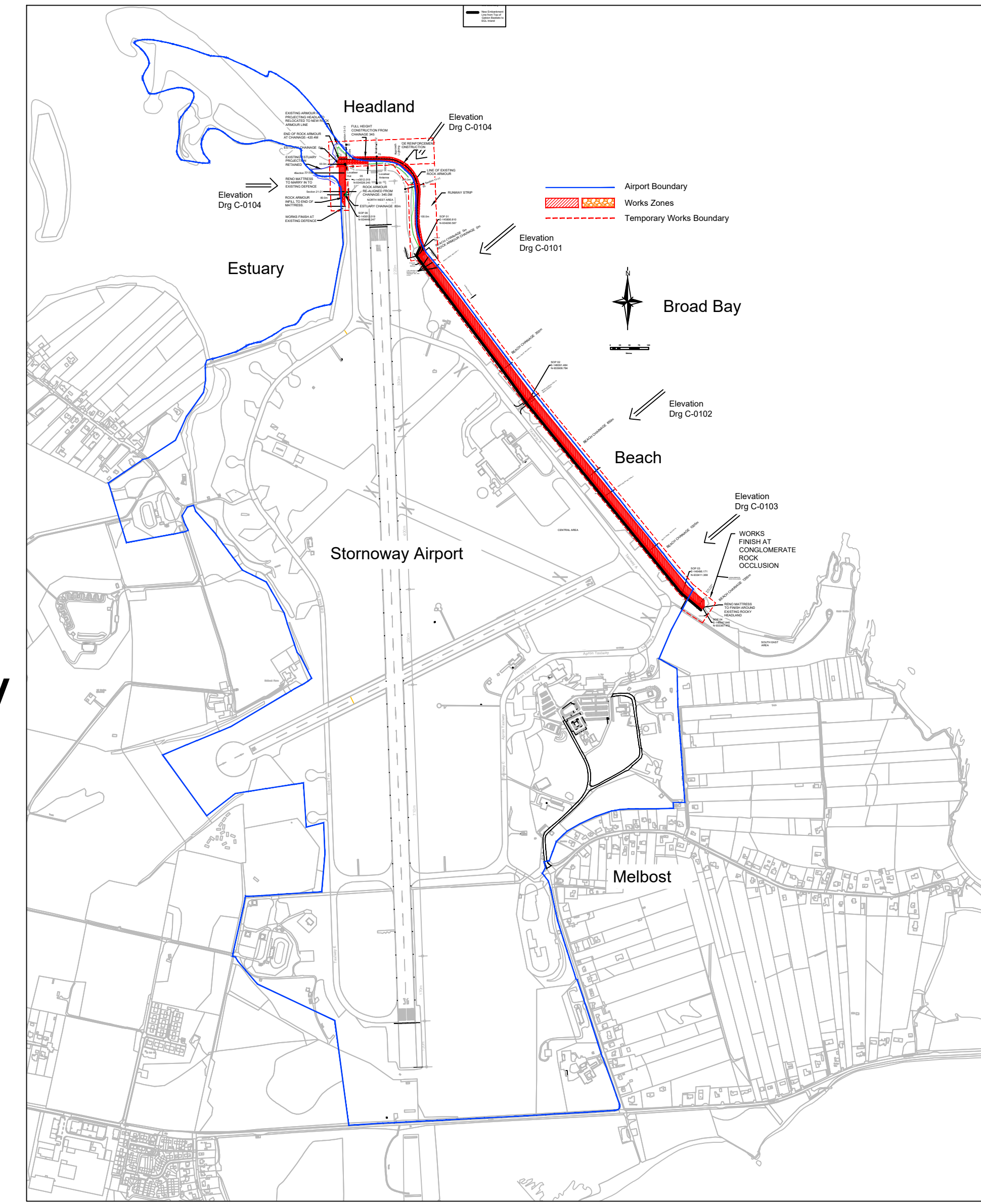
Overall Airport Plan Scale 1:10000
