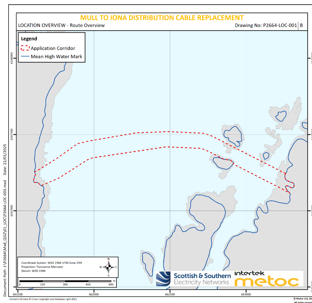
Figure 1-1 Mull to Iona Cable Installation Application Corridor
