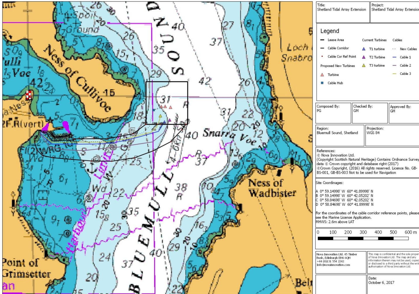
Figure 1 – Nova Innovations Ltd Project Location showing Licence Boundary and Turbine Layout at the Shetland Tidal Array Site, Bluemull Sound, Shetland
