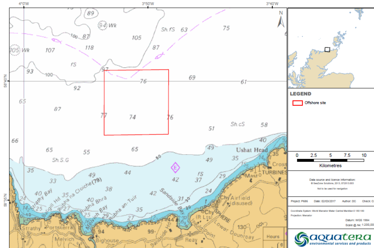
Figure Dounreay Trì Floating Wind Demonstration Project, 6 km off Dounreay, Caithness, North coast of Scotland
