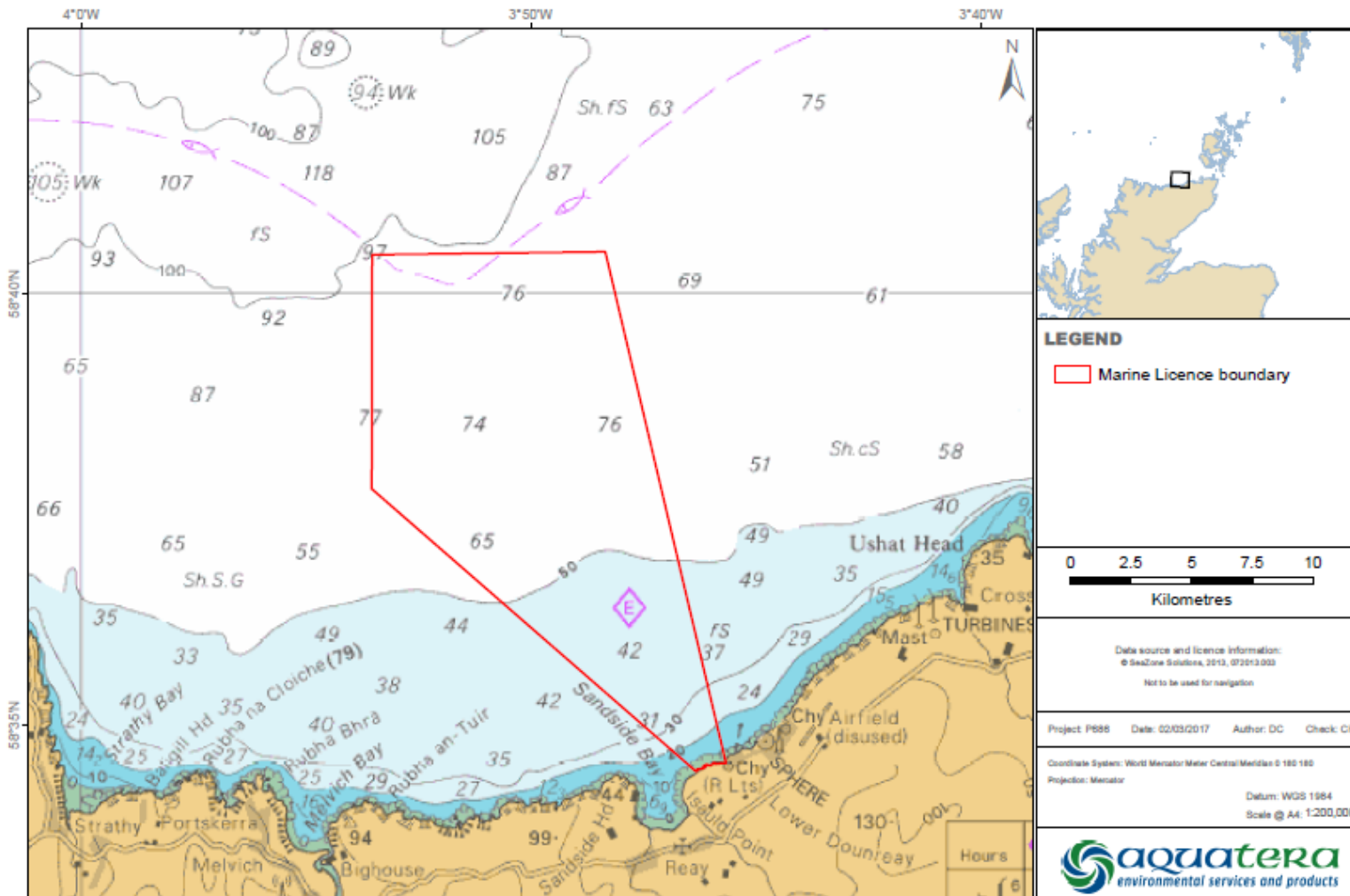
Figure Douvreay Trì Floating Wind Demonstration Project, Cable corridor.
