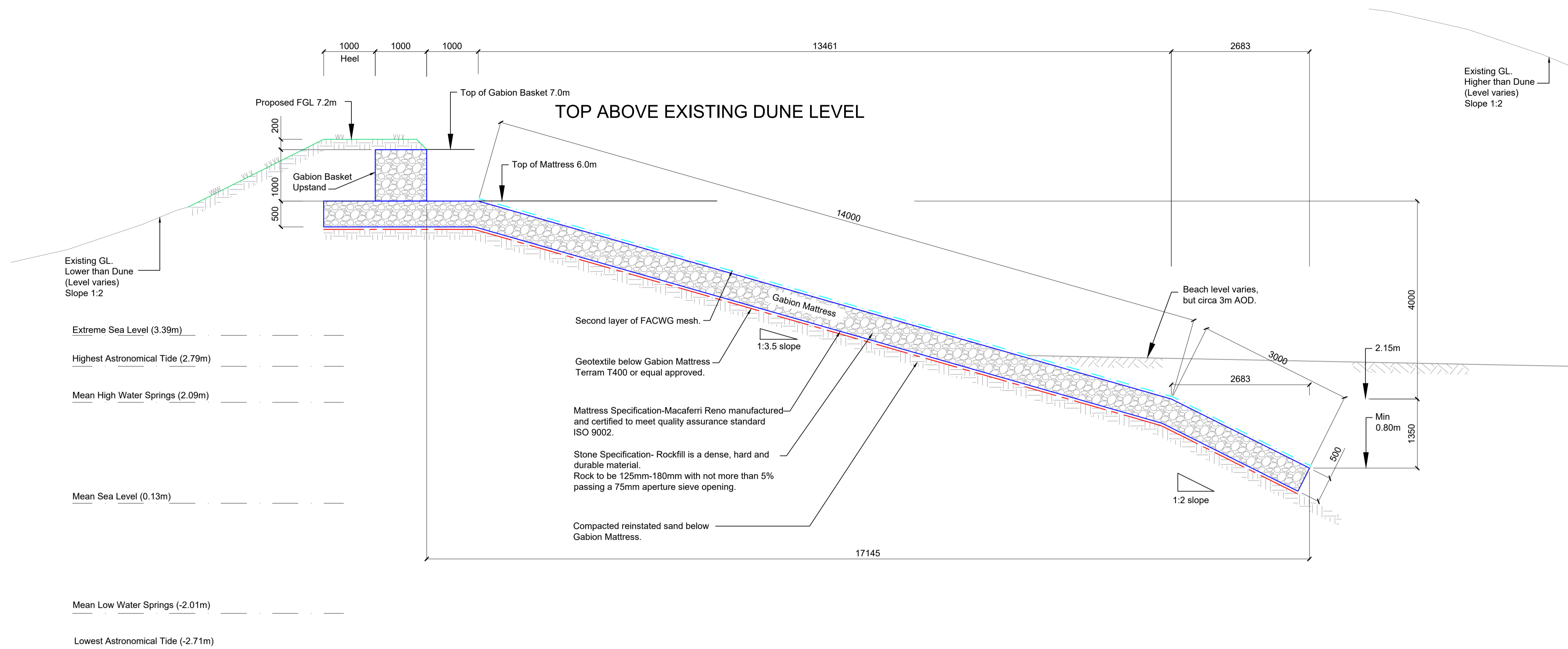
TYPICAL CROSS SECTION CONSTRUCTION DETAIL ALONG BEACH
