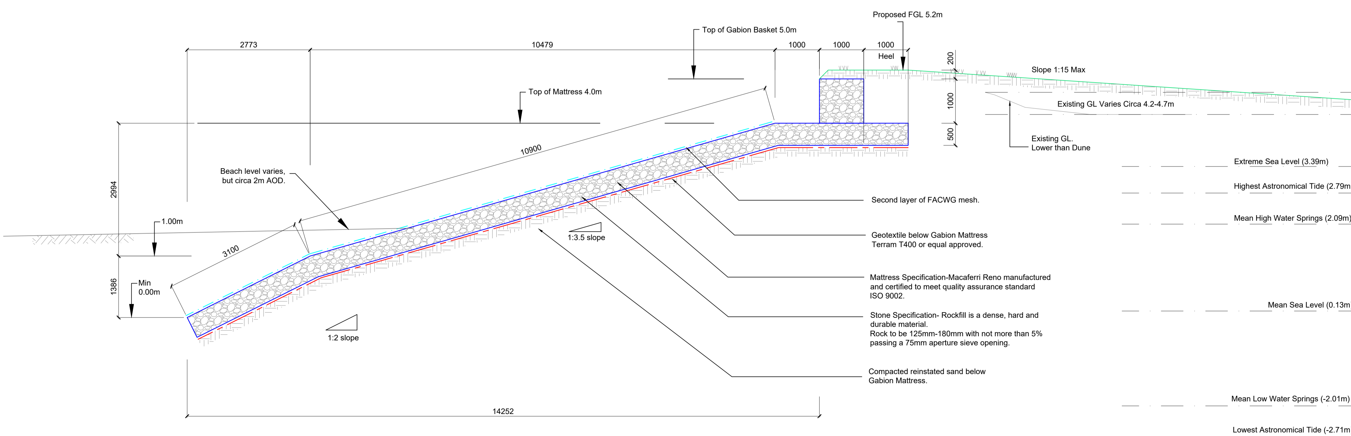
TYPICAL CROSS SECTION CONSTRUCTION DETAIL ALONG ESTUARY
