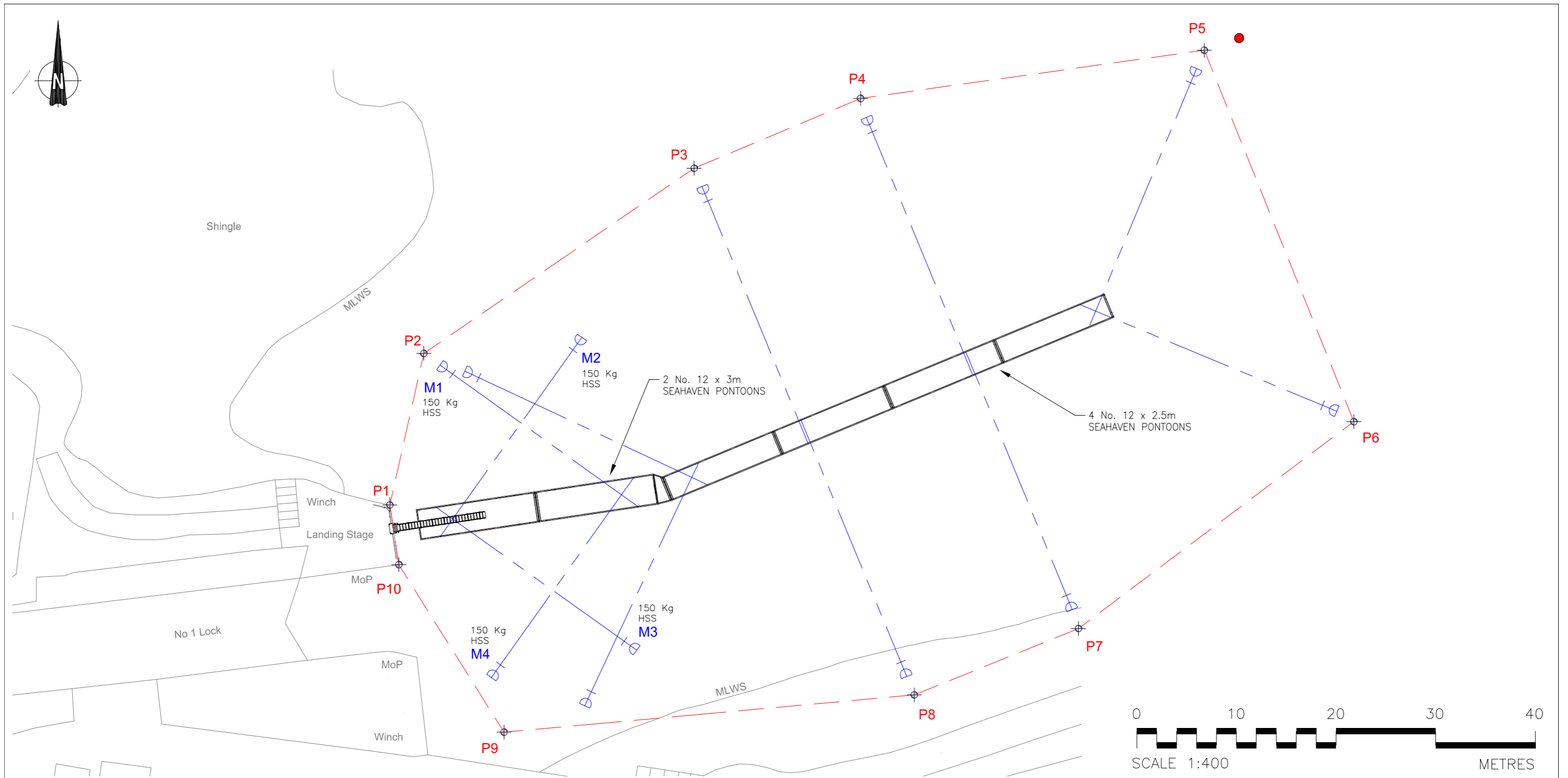
PROPOSED PONTOON MOORING LAYOUT
