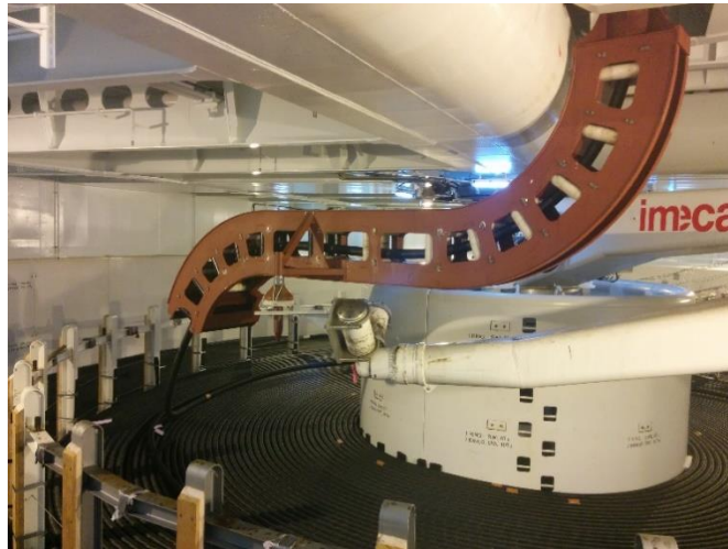
Figure 5-19: Partitioned carousel with cable loading
