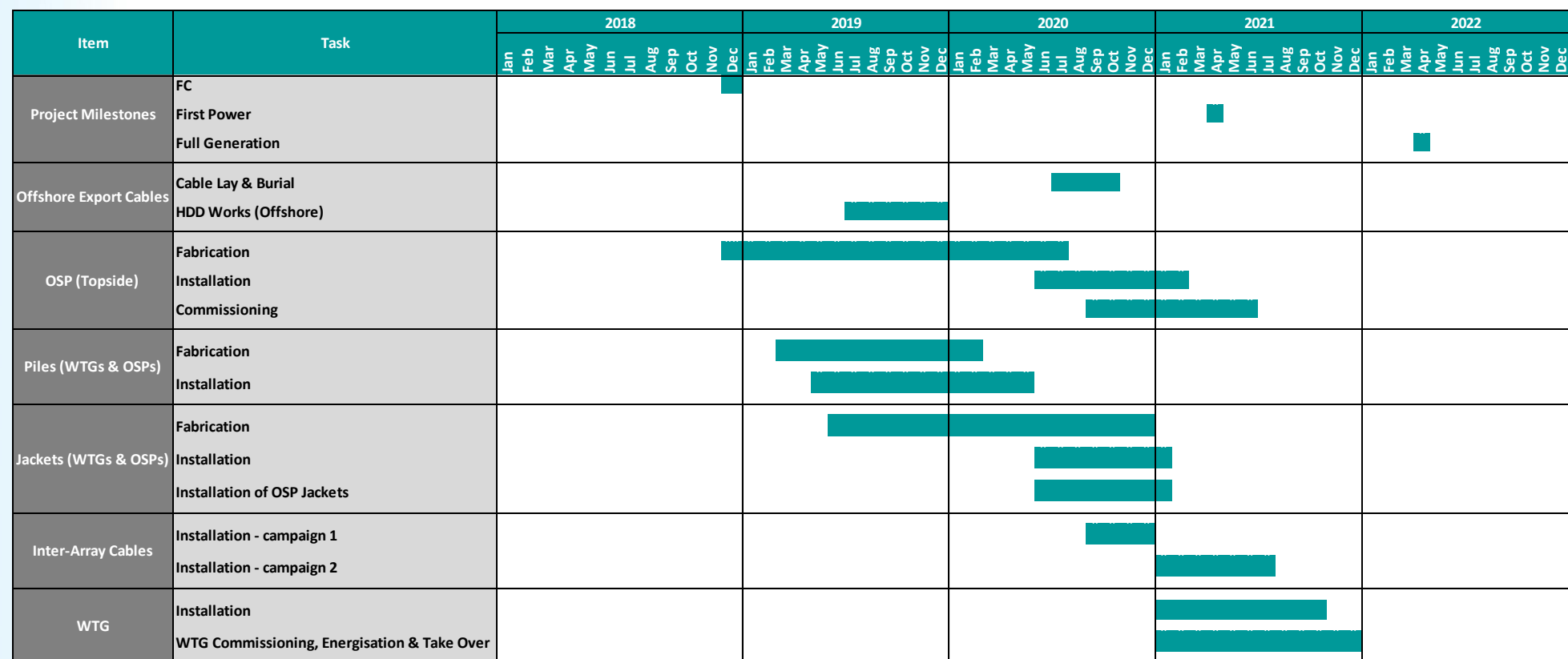
Figure 4-1: Offshore Construction Programme
