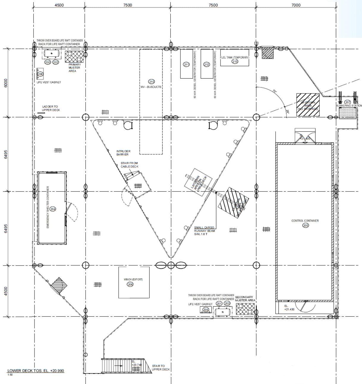
Figure 4-4: OSP general arrangement – plan view of topside lower deck
