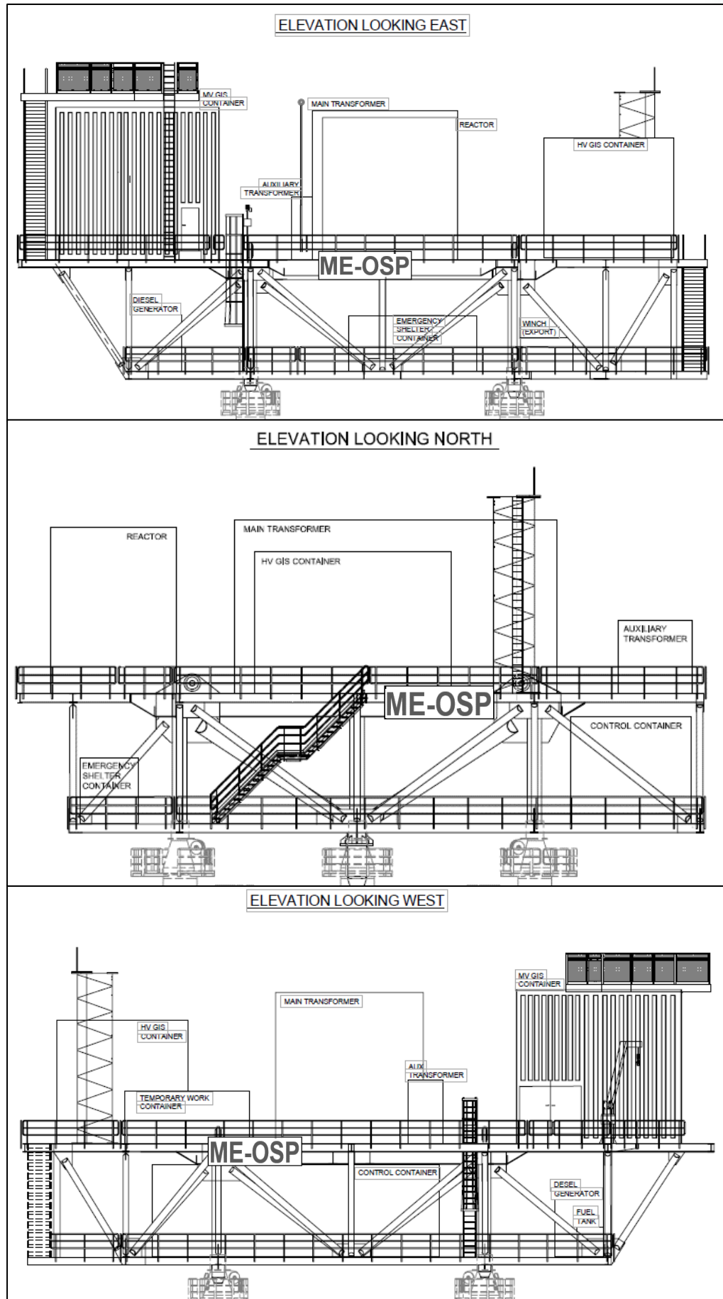
Figure 4-2: OSP general arrangement of topside – side elevation, end elevation and reverse side elevation
