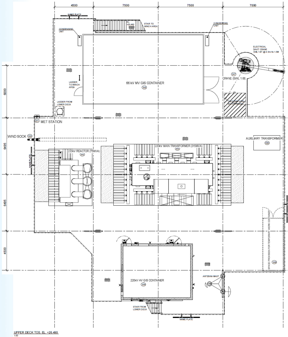
Figure 4-3: OSP general arrangement – plan view of topside upper deck
