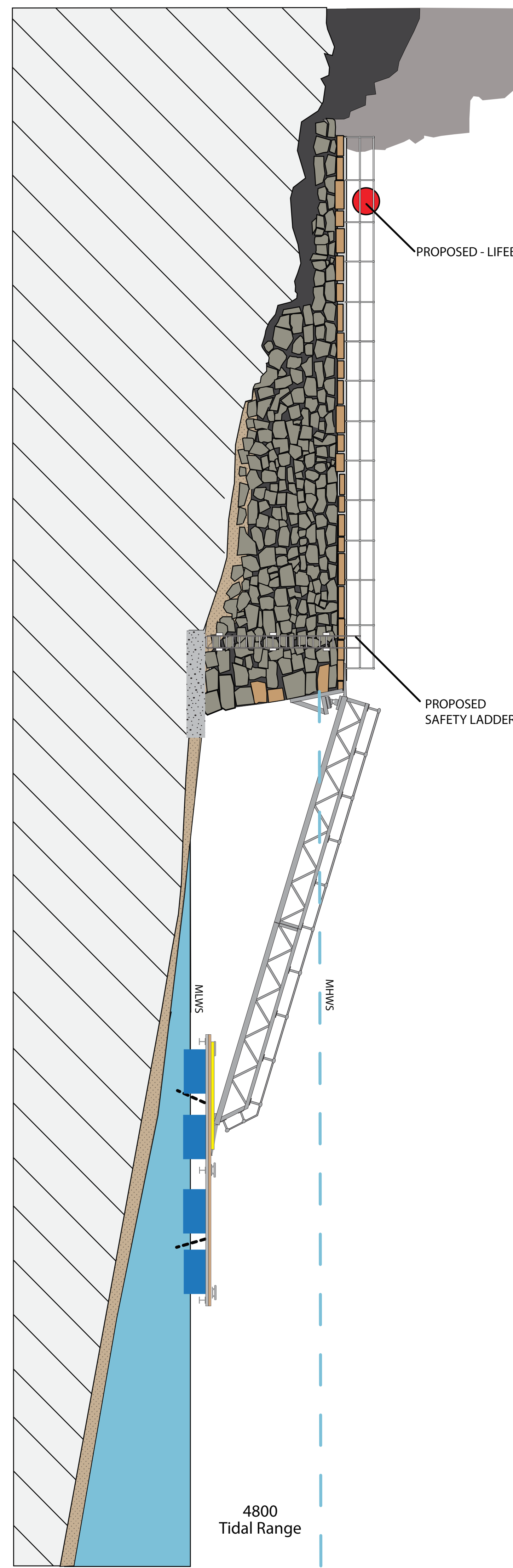
NORTH FACE OF PIER PONTON SUPPORT, BRIDGE AND PONTON VIEW SOUTH FROM SECTION A A
