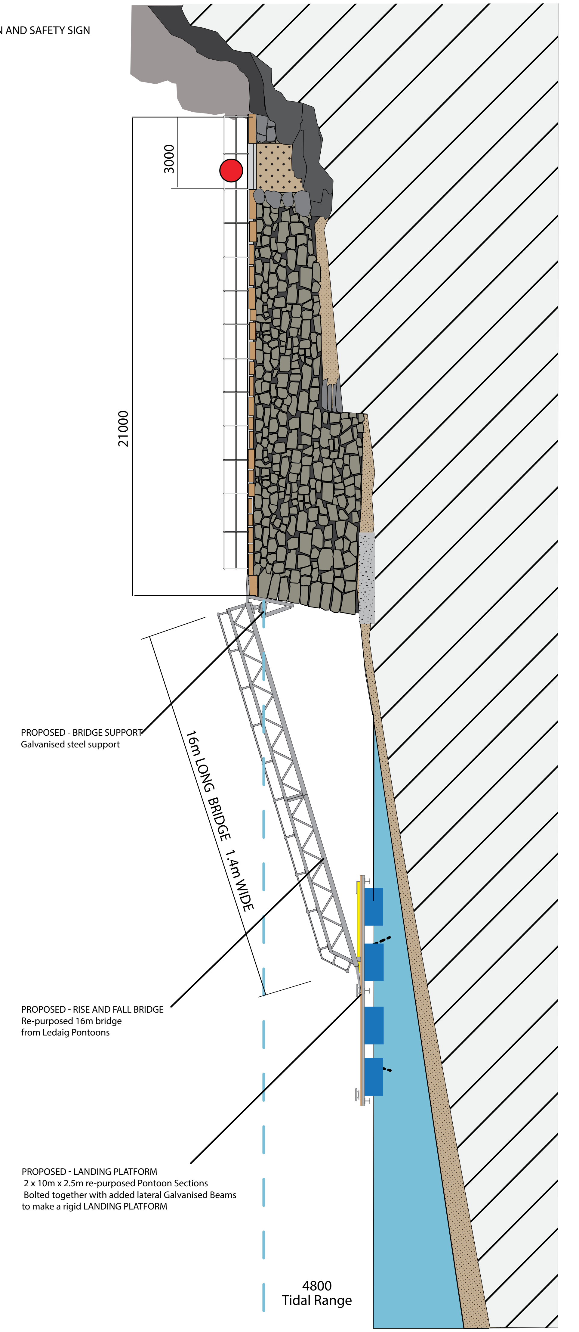
SOUTH FACE OF PIER PONTON SUPPORT, BRIDGE AND PONTON VIEW NORTH FROM SECTION B B
