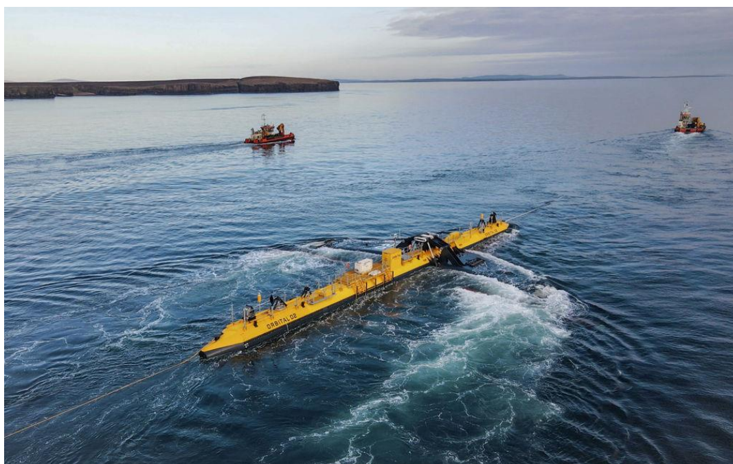
Figure 5: Indicative tow arrangement for O2.4 device (Source: Orbital Marine Power).
