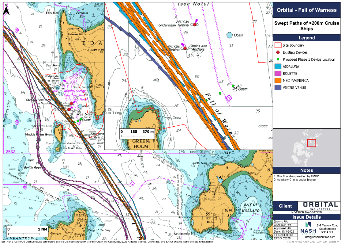
Figure 19: Swept Paths of >200m Cruise Ships.
