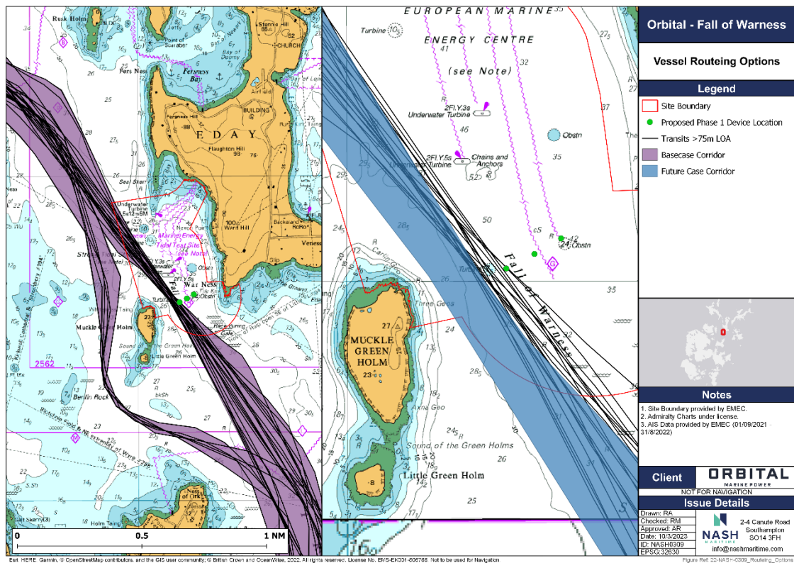
Figure 20: Vessel Routing Options.
