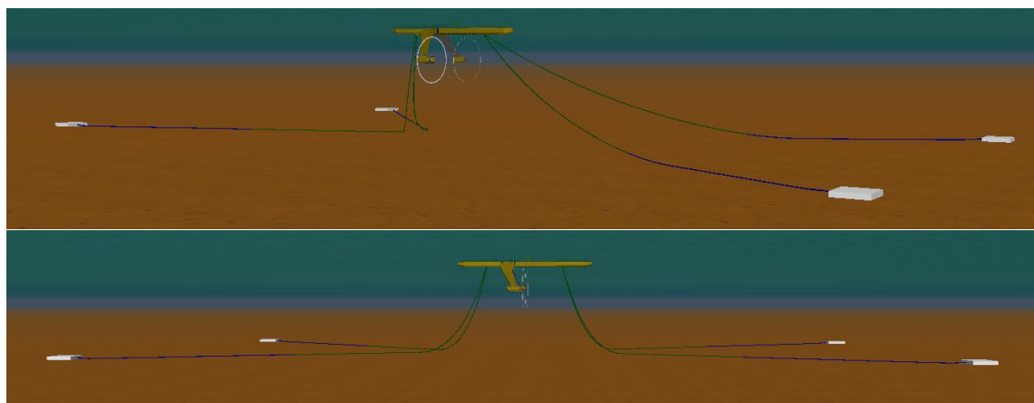
Figure 3: Orbital O2.4 mooring system.
