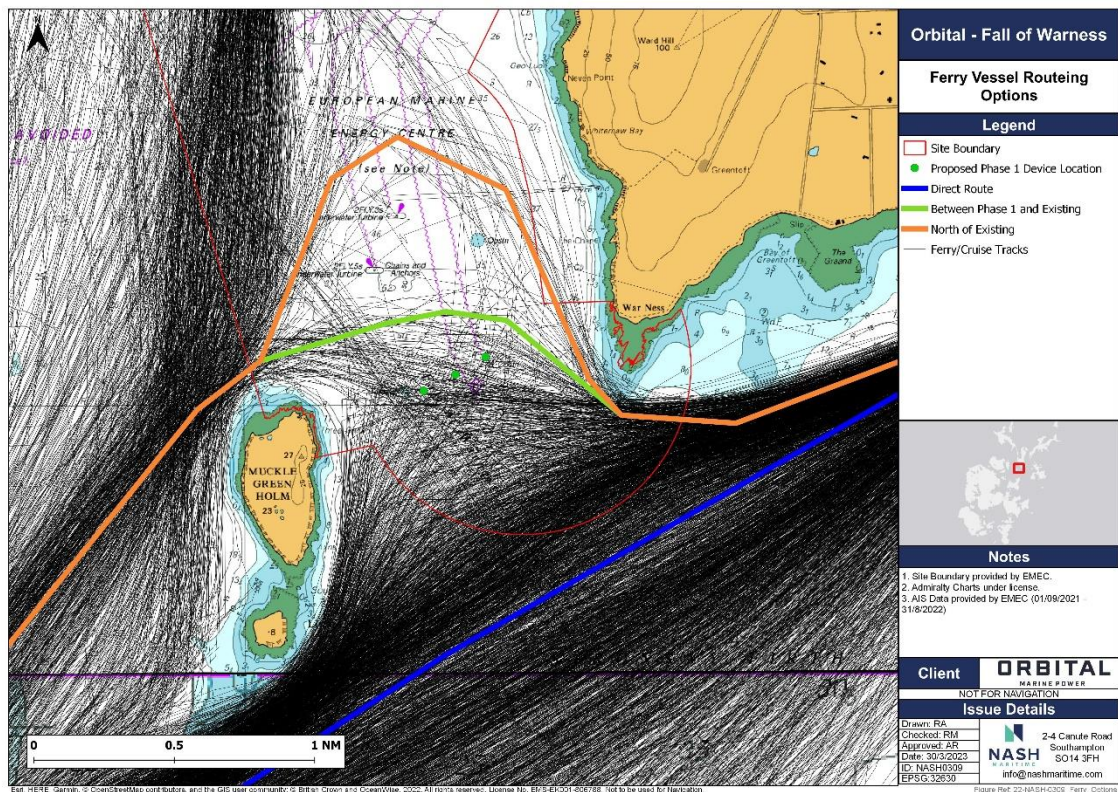
Figure 23: Alternative routes with Devices in Position.
