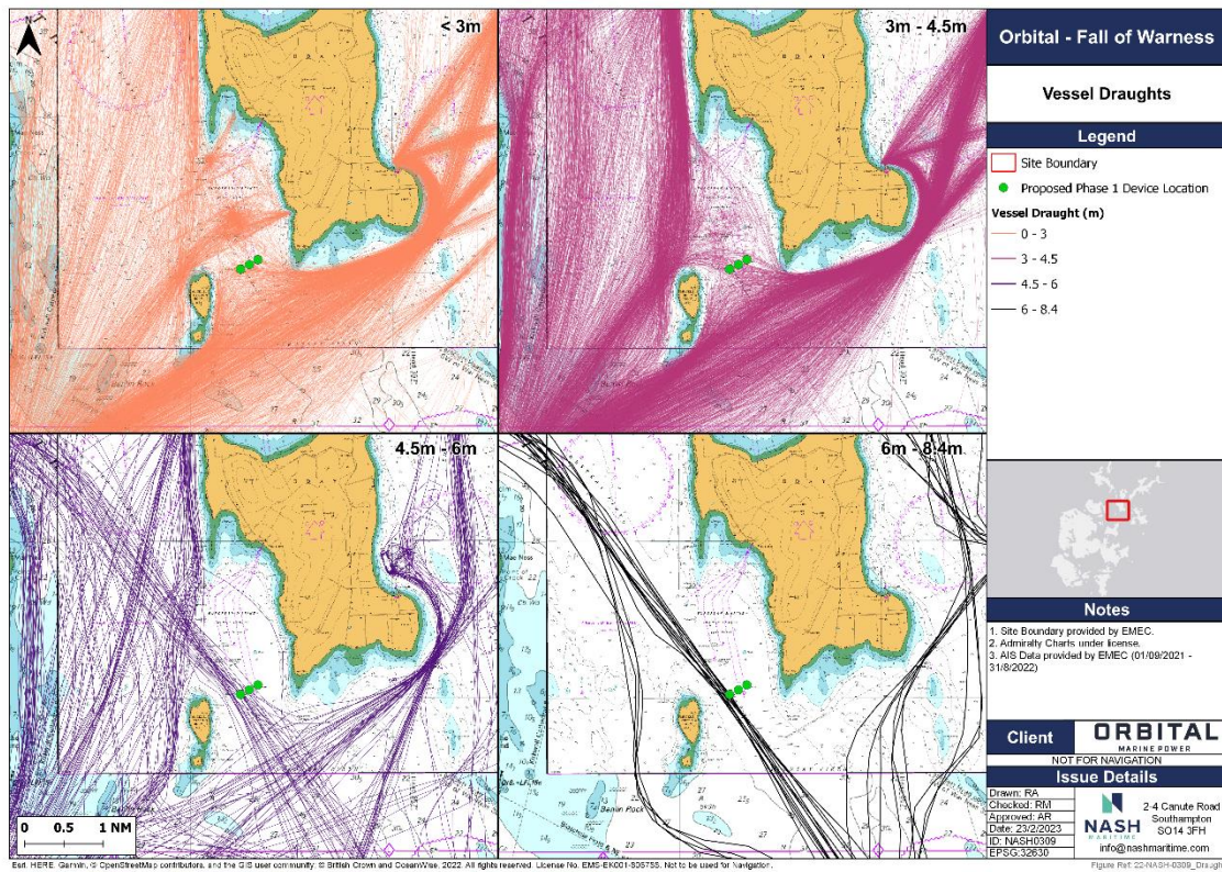
Figure 9: Vessel Tracks by Draught (metres).
