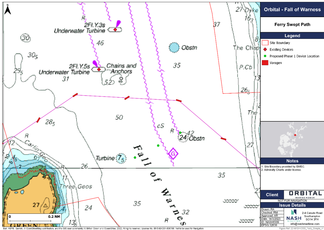
Figure 22: Swept path of Varagen to scale (08:00 15/05/2022).
