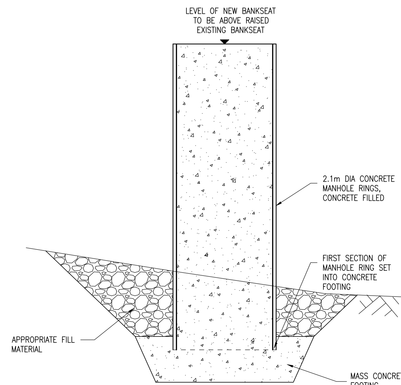
SECTION THROUGH NEW BANKSEAT (SCALE 1:50)
