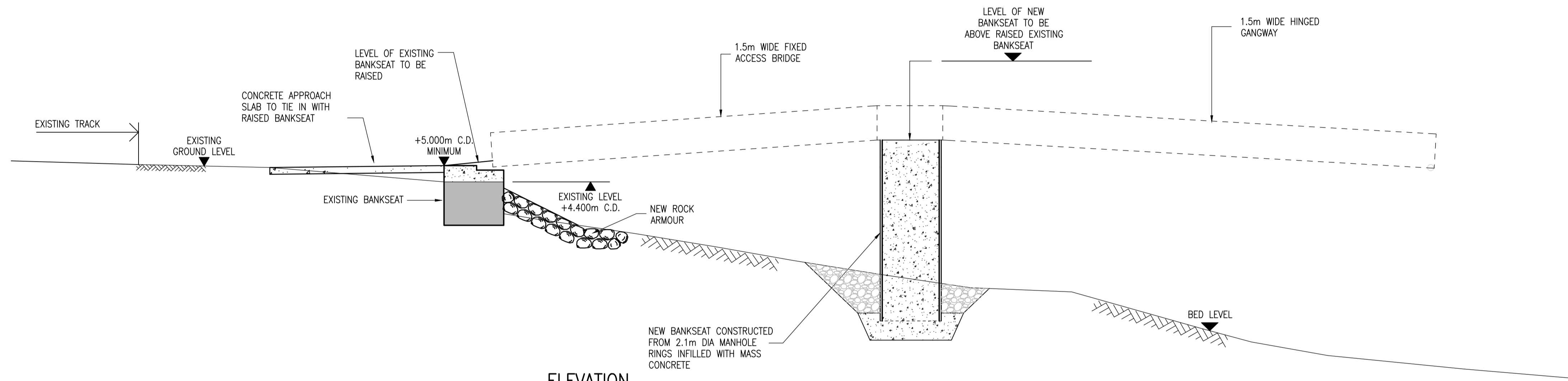
ELEVATION (SCALE 1:250)
