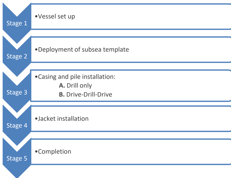
Figure 3-1: Pile foundation (and jacket substructure) installation sequence.
