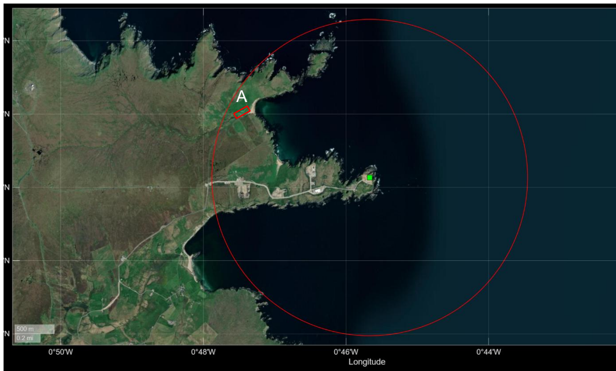
Figure 2 Ground Launch Exclusion Zone suggested by the FSA of HyImpulse
