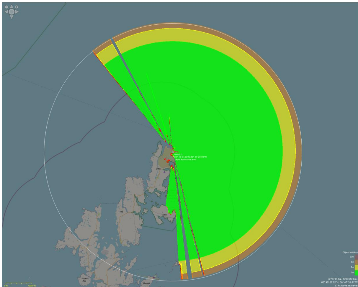
Figure 6 Maritime radar and camera system coverage
