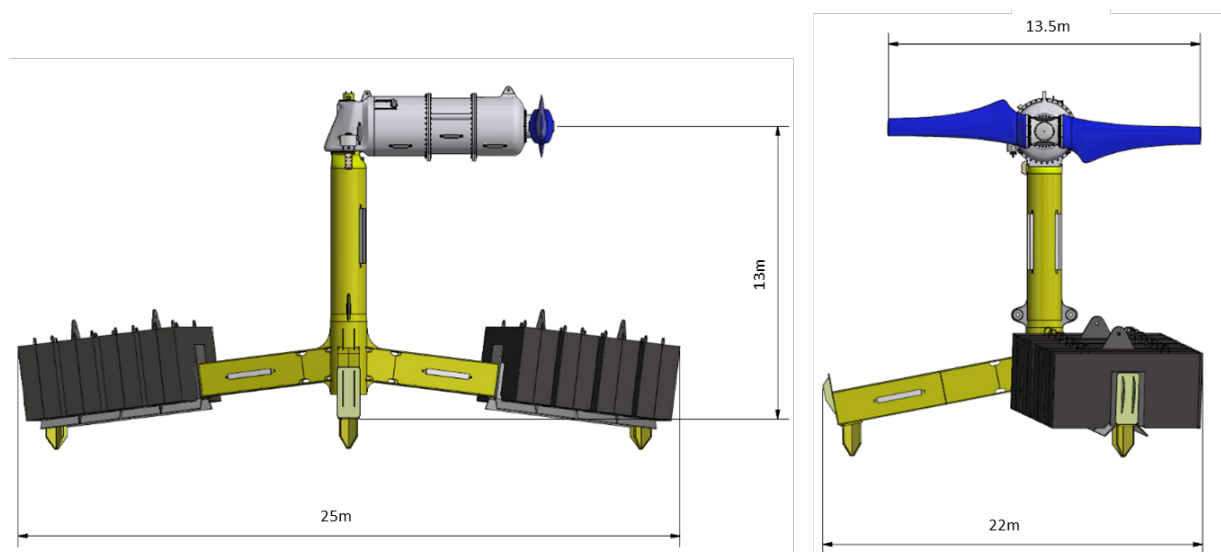
Figure 4. Dimensions of Nova's Oceanstar turbine.
