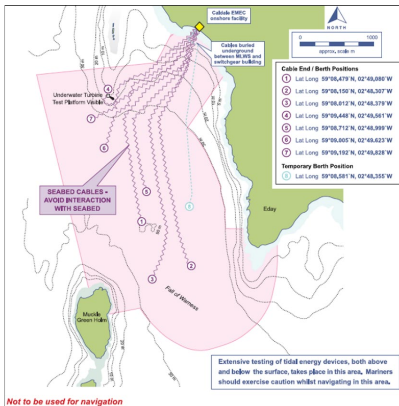
Figure 2. EMEC Fall of Warness site.
