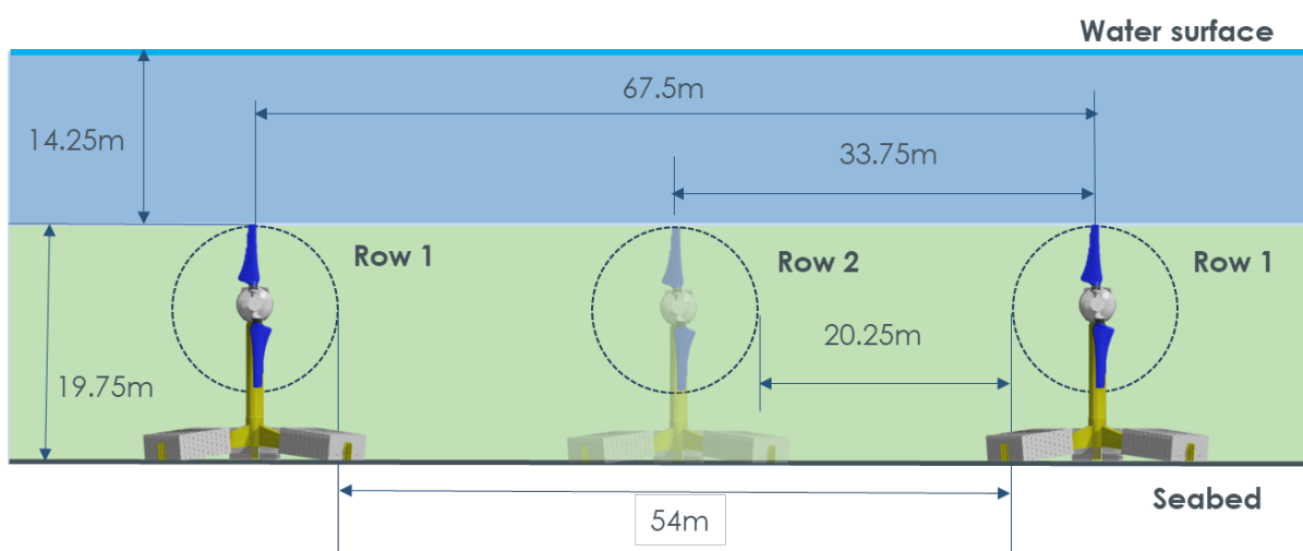
Figure 6. Front elevation profile of the array viewed from the north. Copyright © Nova Innovation 2023
