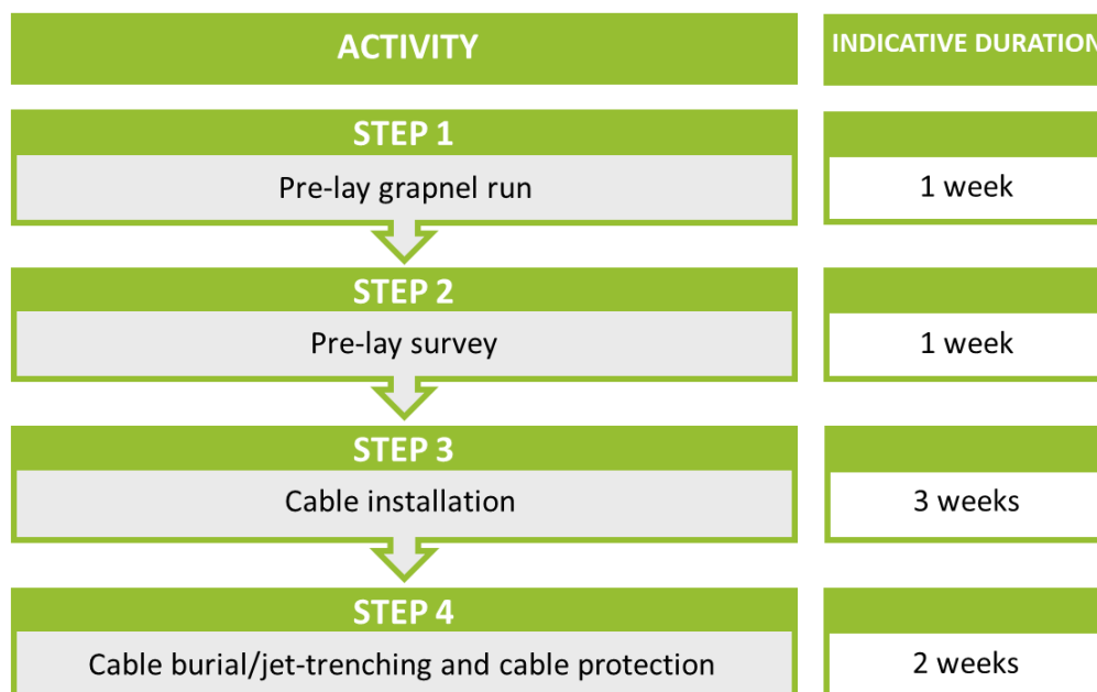
Figure 6.9: Overview of OSP interconnection cable installation process.
