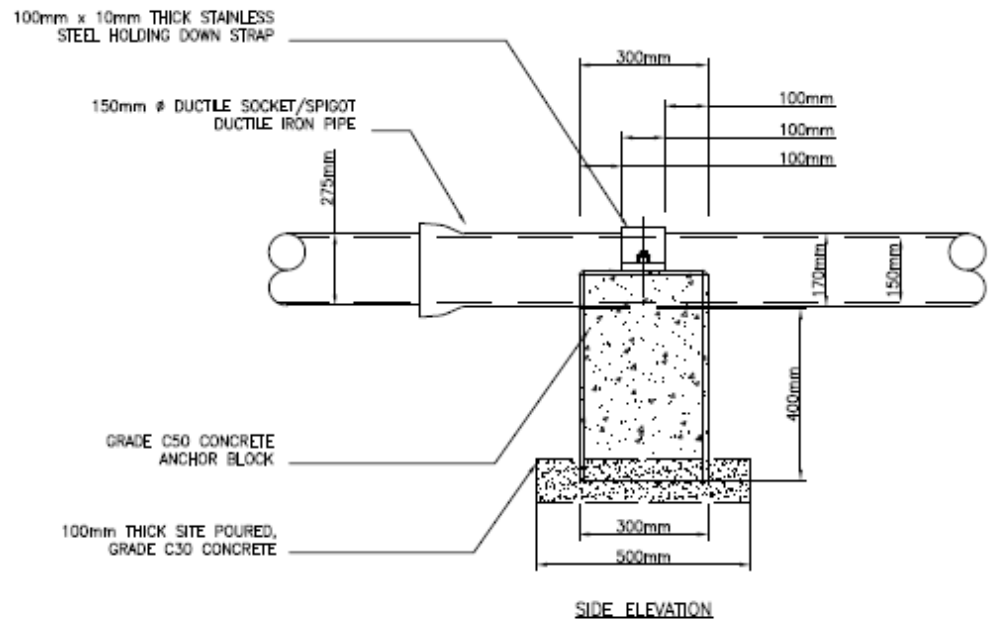
DUCTILE IRON PIPE OUTFALL SUPPORTS SCALE 1:10
