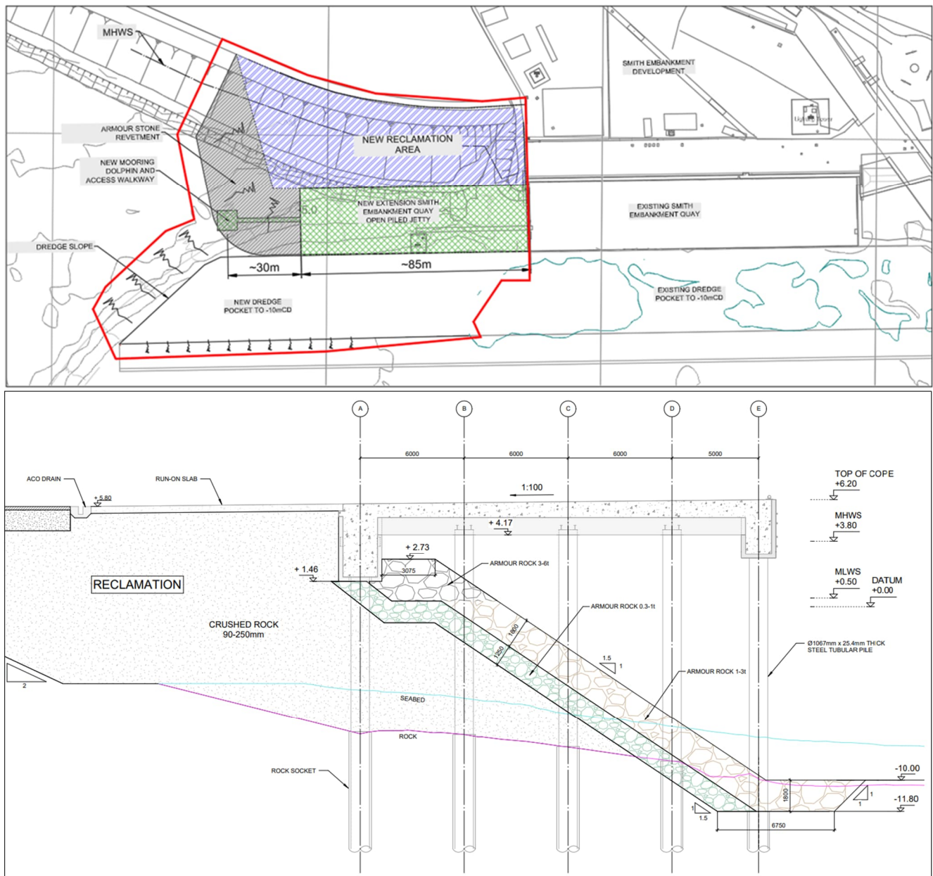
Figure 4.1 Proposed extension of Smith Quay.
