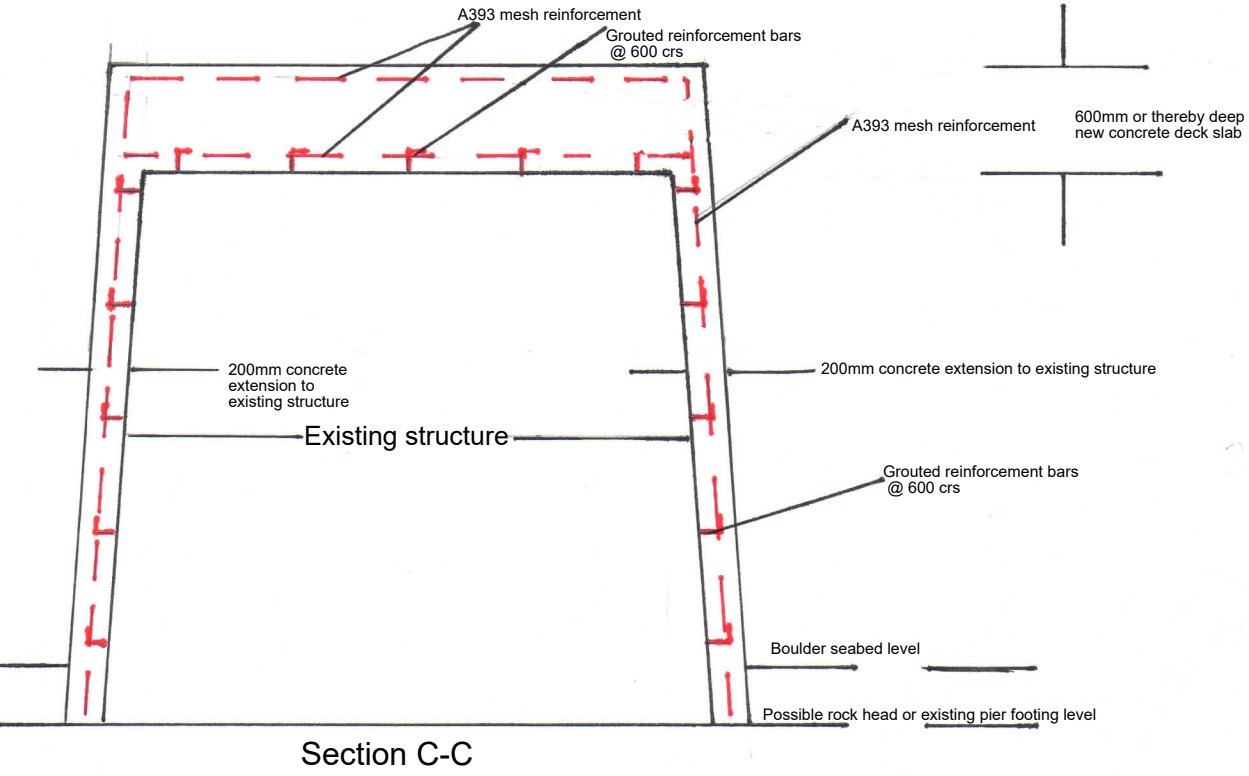
Culkein Pier Sections Scale 1:40
