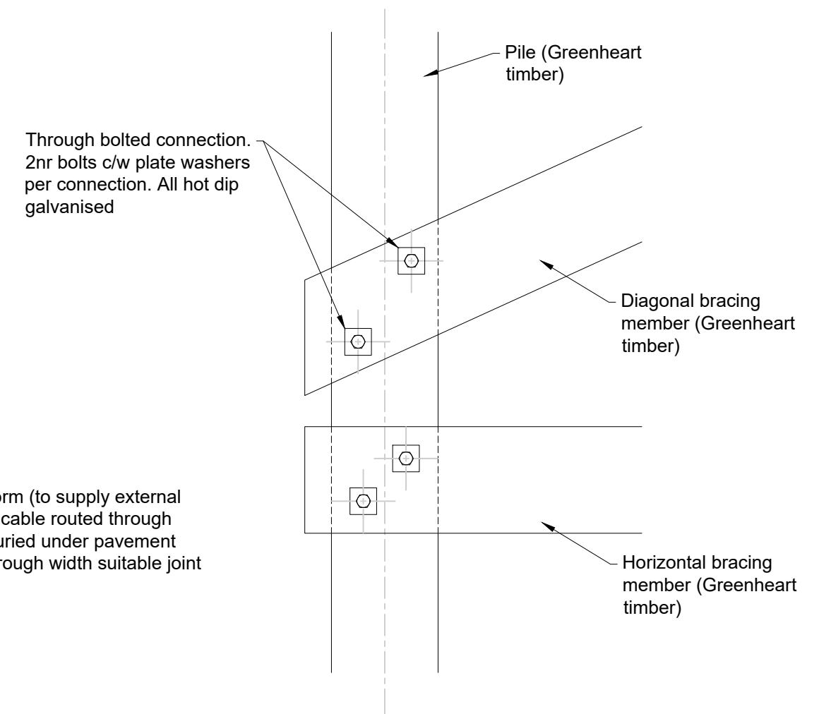
Framing Connection Detail (Typical) Scale 1:10
