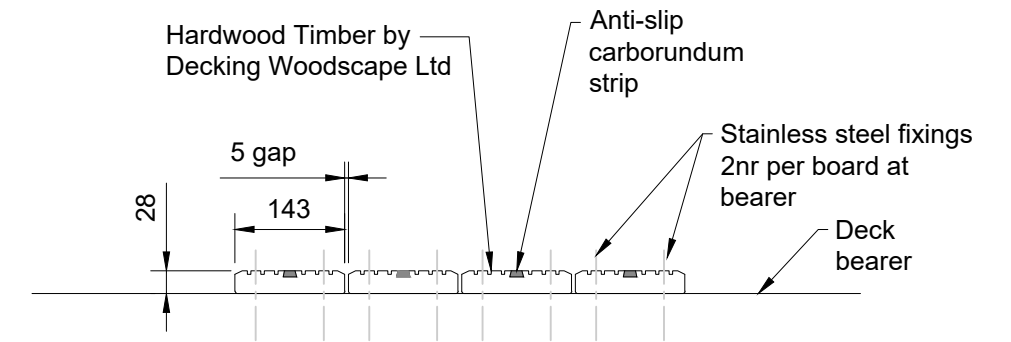
Platform Decking Detail (Typical) Scale 1:10
