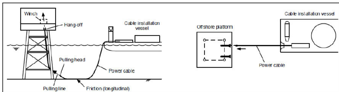
Figure 7-2 Typical 1st end pull-in operation
