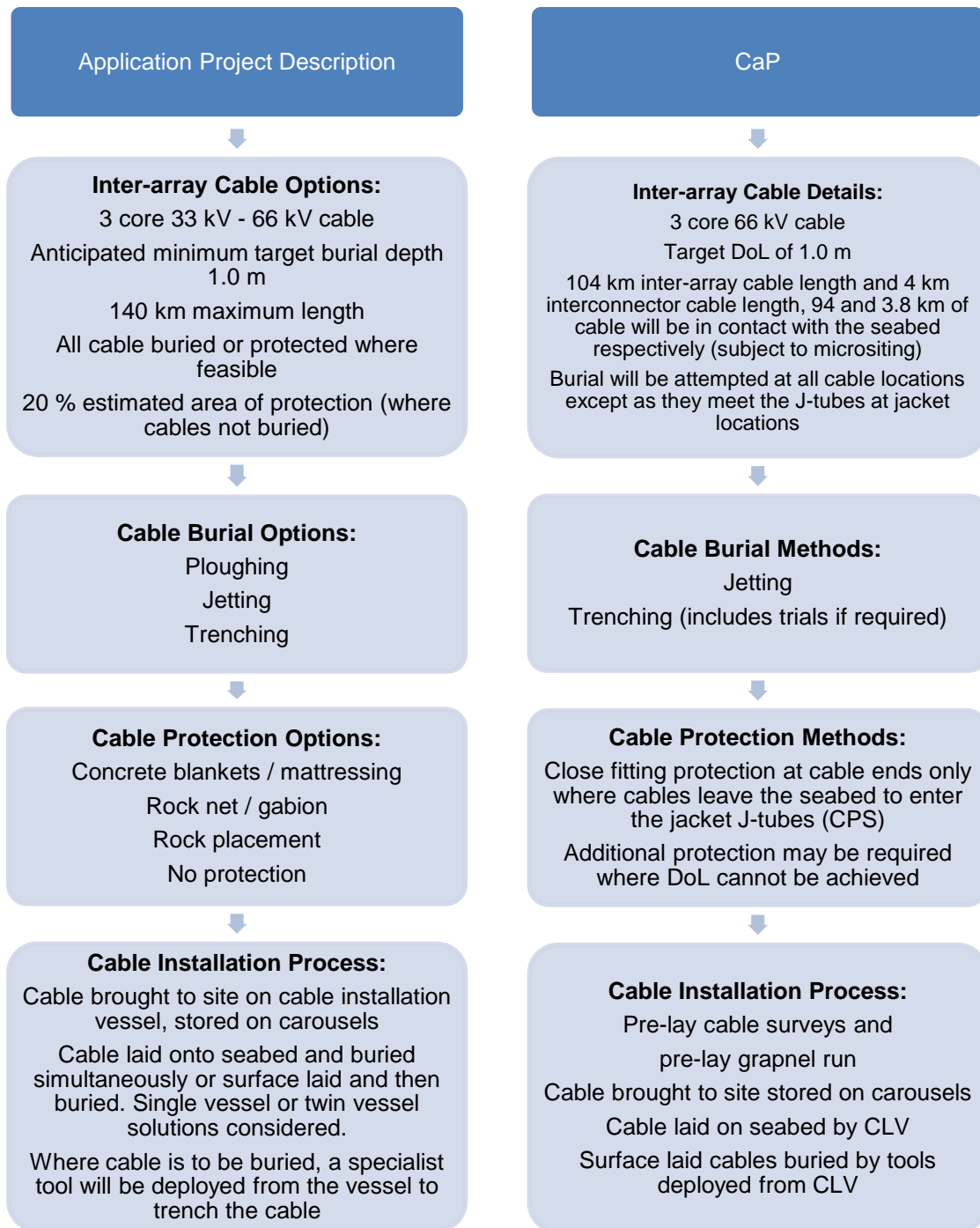
Figure 9-1: Comparison of inter-array and interconnector cable installation methods described in the Application and CaP
