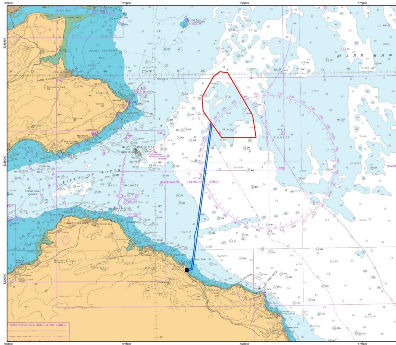
Figure 3-1: Wind Farm Area and Offshore Export Cable Corridor locations
