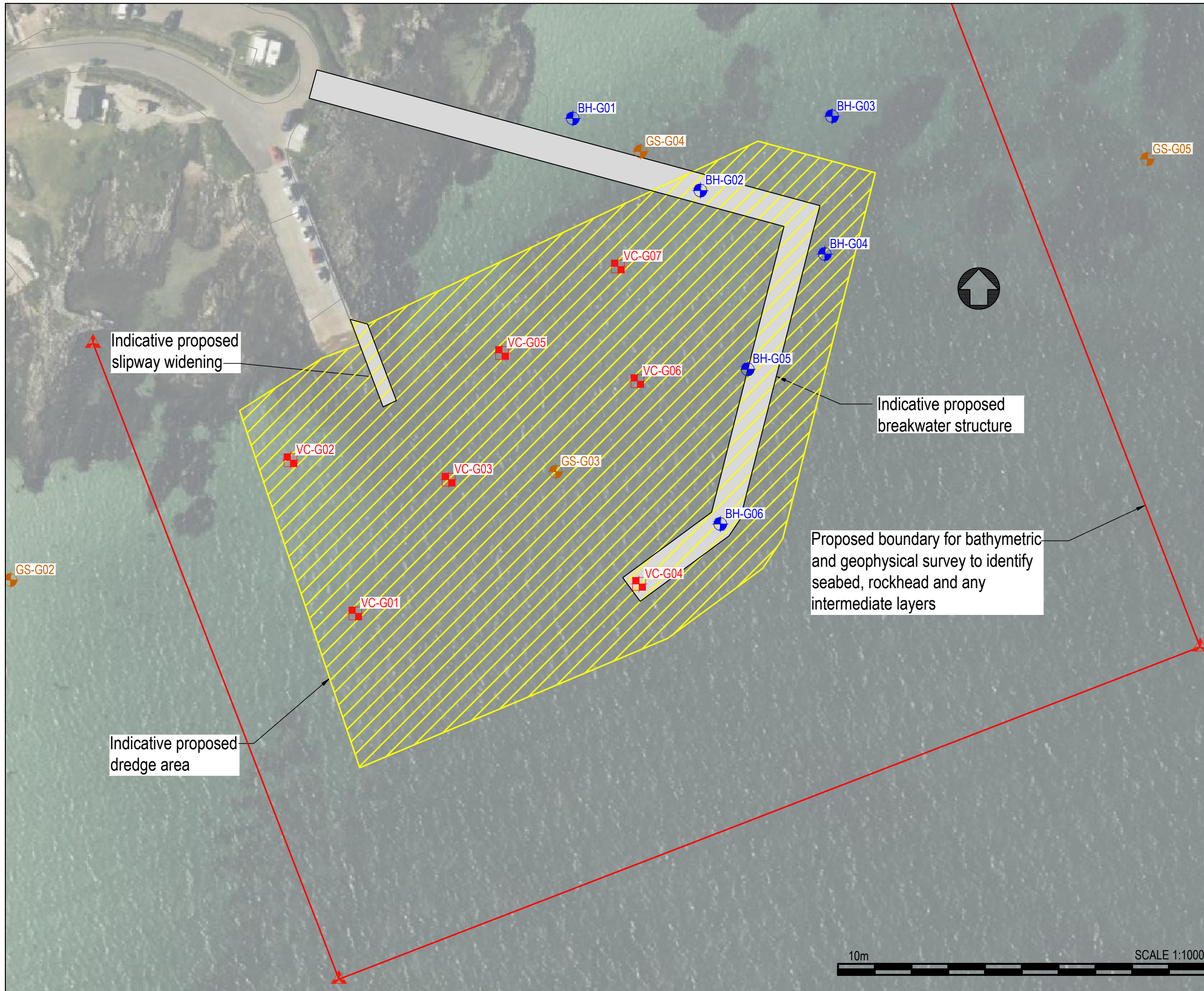
Proposed Ground Investigation and Geophysical Works Layout [1:1000]
