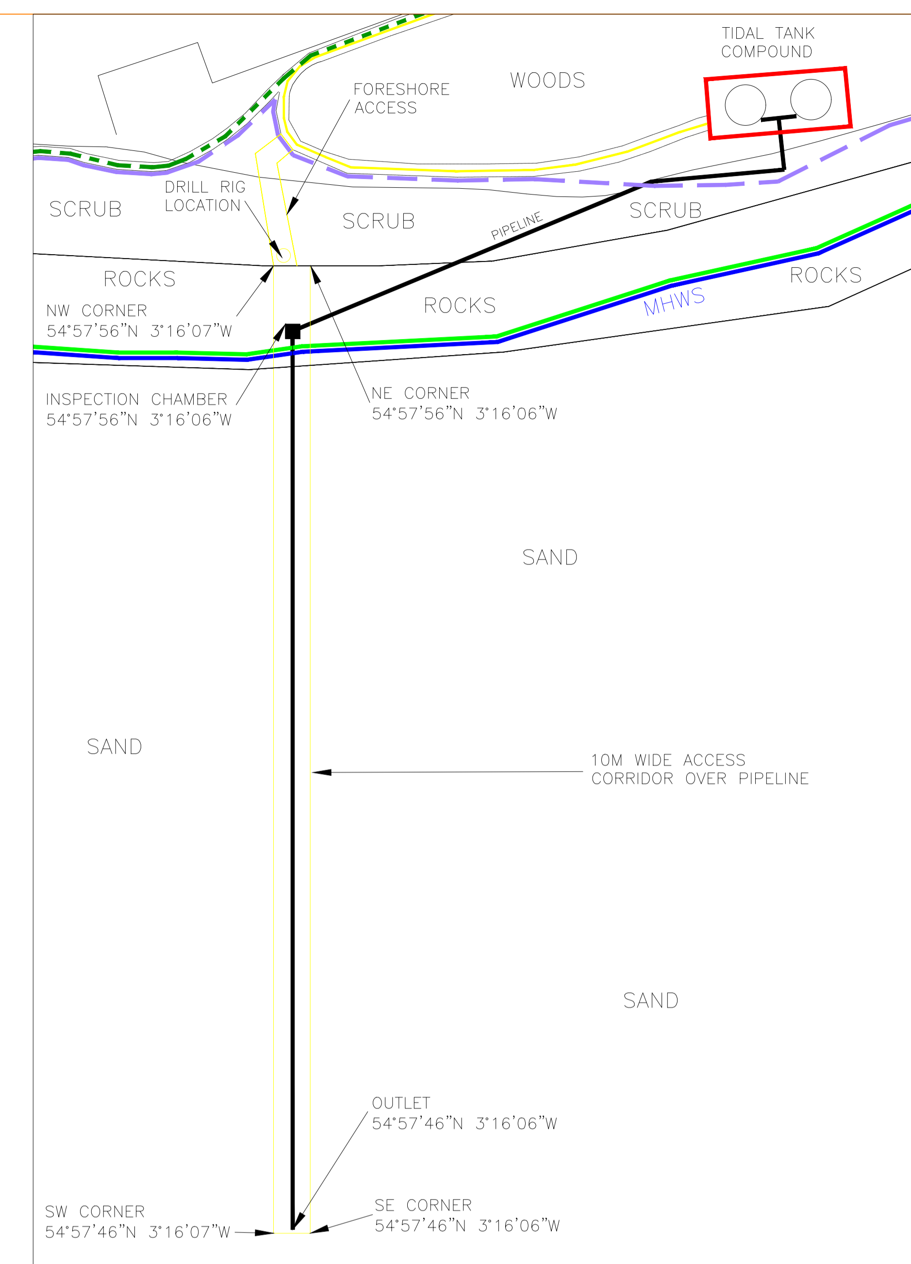
DETAIL 1 - OUTLET PIPEWORK (SCALE 1:1000)
