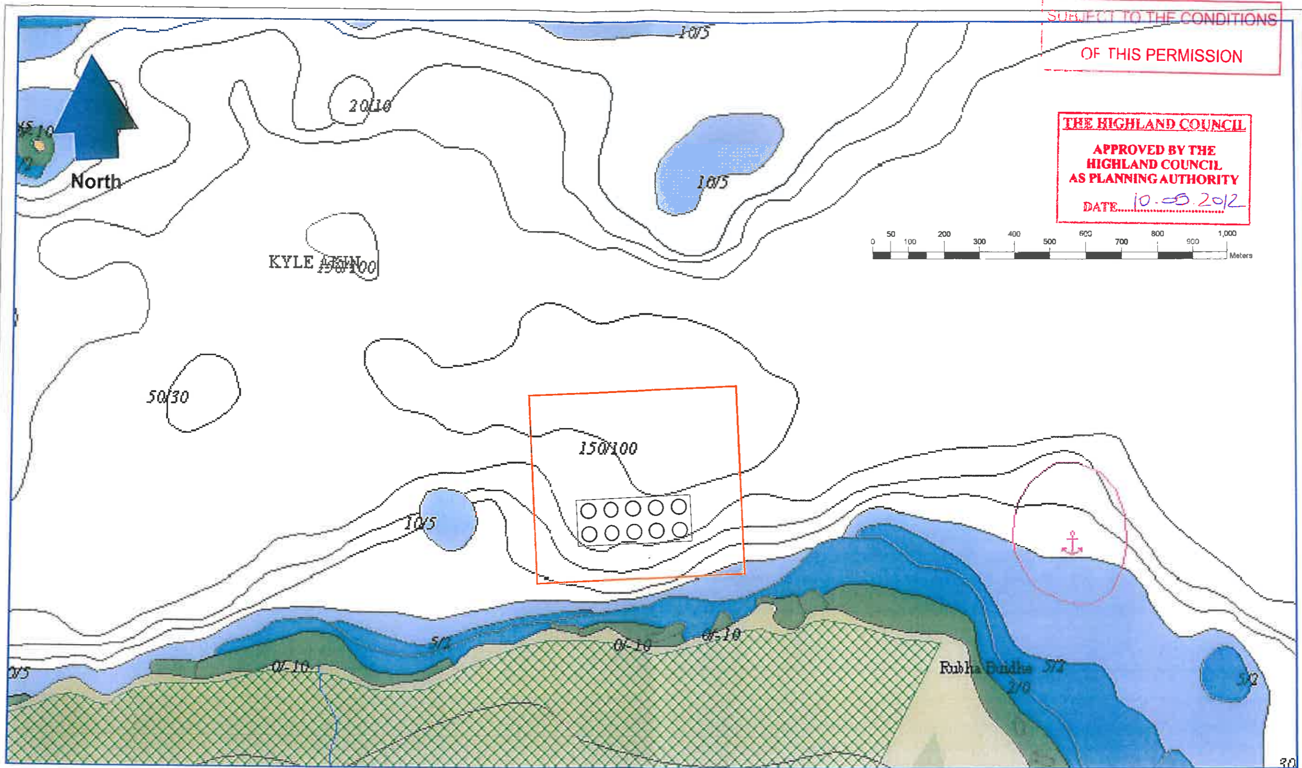
SRON: LOCH ALSH, KYLE OF LOCHALSH ADMIRALTY CHART EXTRACT OF SITE LOCATION Figure 5 Detailed view of Sron, Loch Alsh proposal. 10 circular plastic cages 120m circumference.
