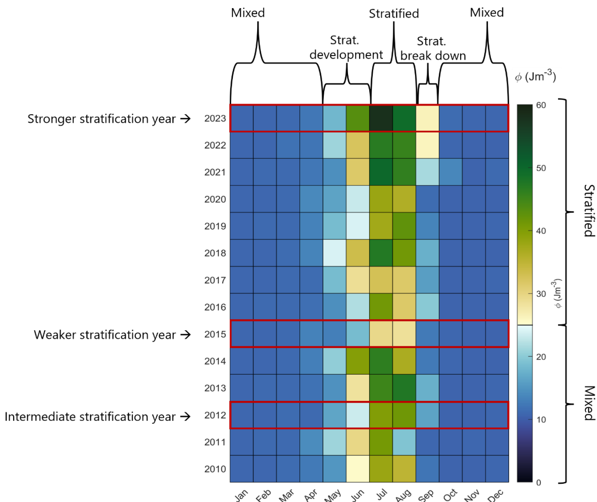
Figure 5.4: Monthly PEA ( \phi ) Values, Based on the Copernicus Reanalysis Monthly Temperature and Salinity Data, in the Array Area from 2010 to 2023
