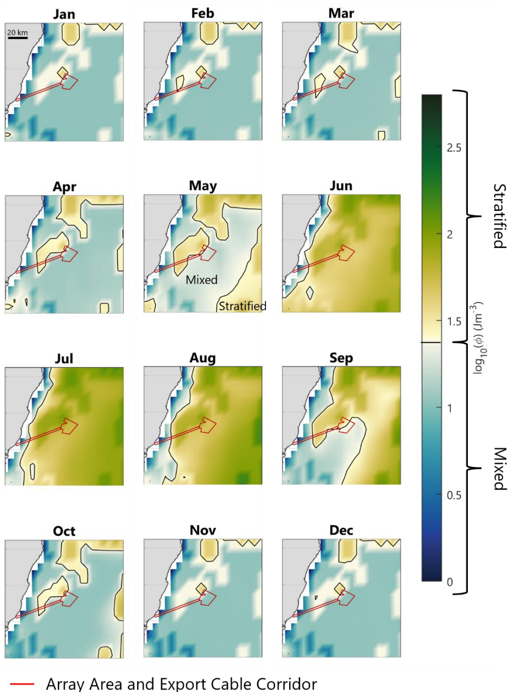
Figure 5.1: Calculated PEA ( \phi ), Based on the Copernicus Reanalysis Monthly Temperature and Salinity Data for 2023, a Stronger Stratification Year
