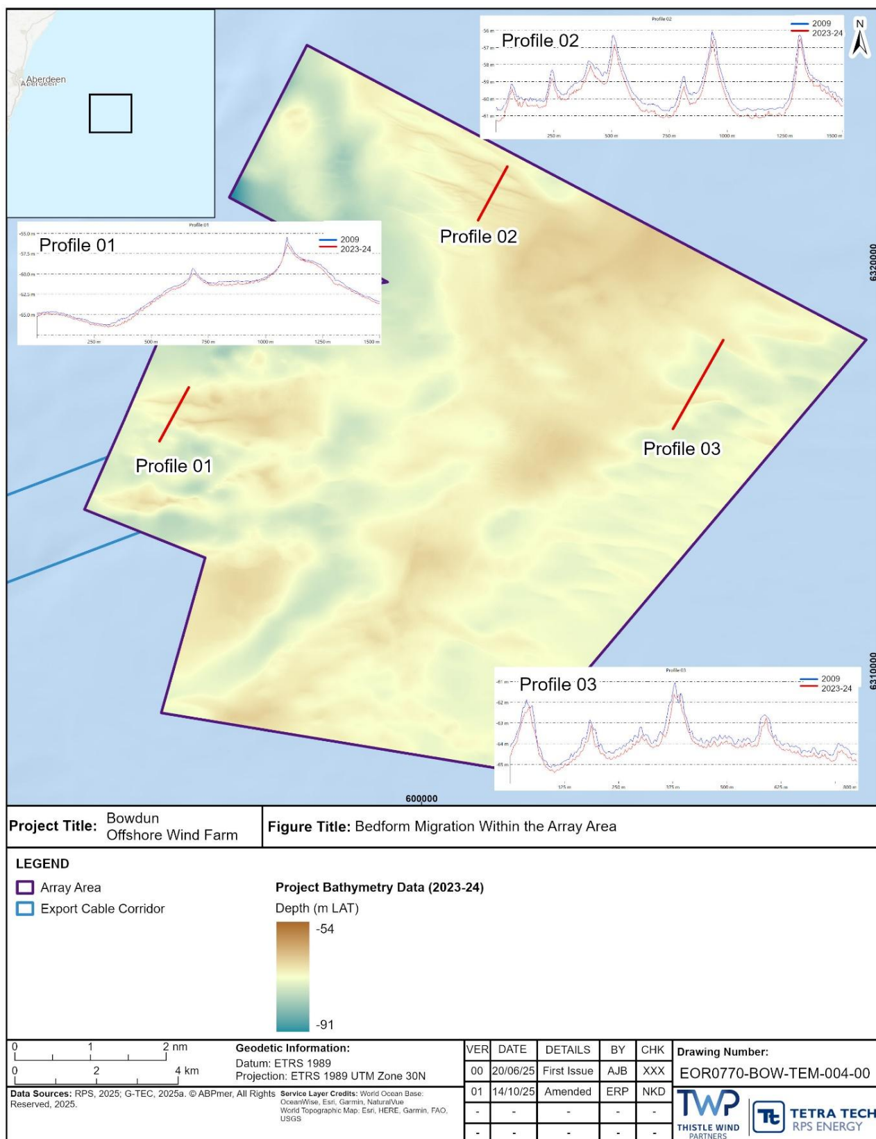
Figure 6.8: Bedform Migration Within the Array Area
