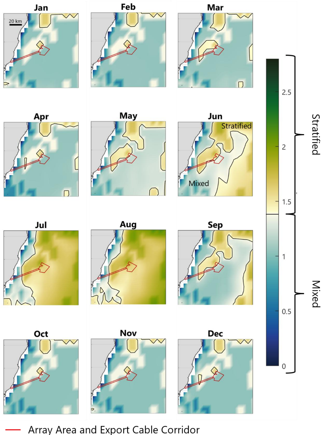
Figure 5.2: Calculated PEA ( \phi ), Based on the Copernicus Reanalysis Monthly Temperature and Salinity Data for 2012, an Intermediate Stratification Year
