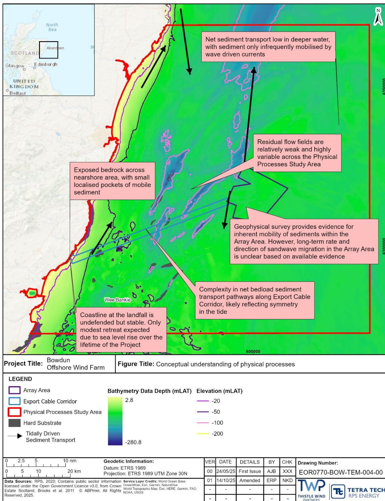
Figure 6.4: Conceptual Understanding of Physical Processes
