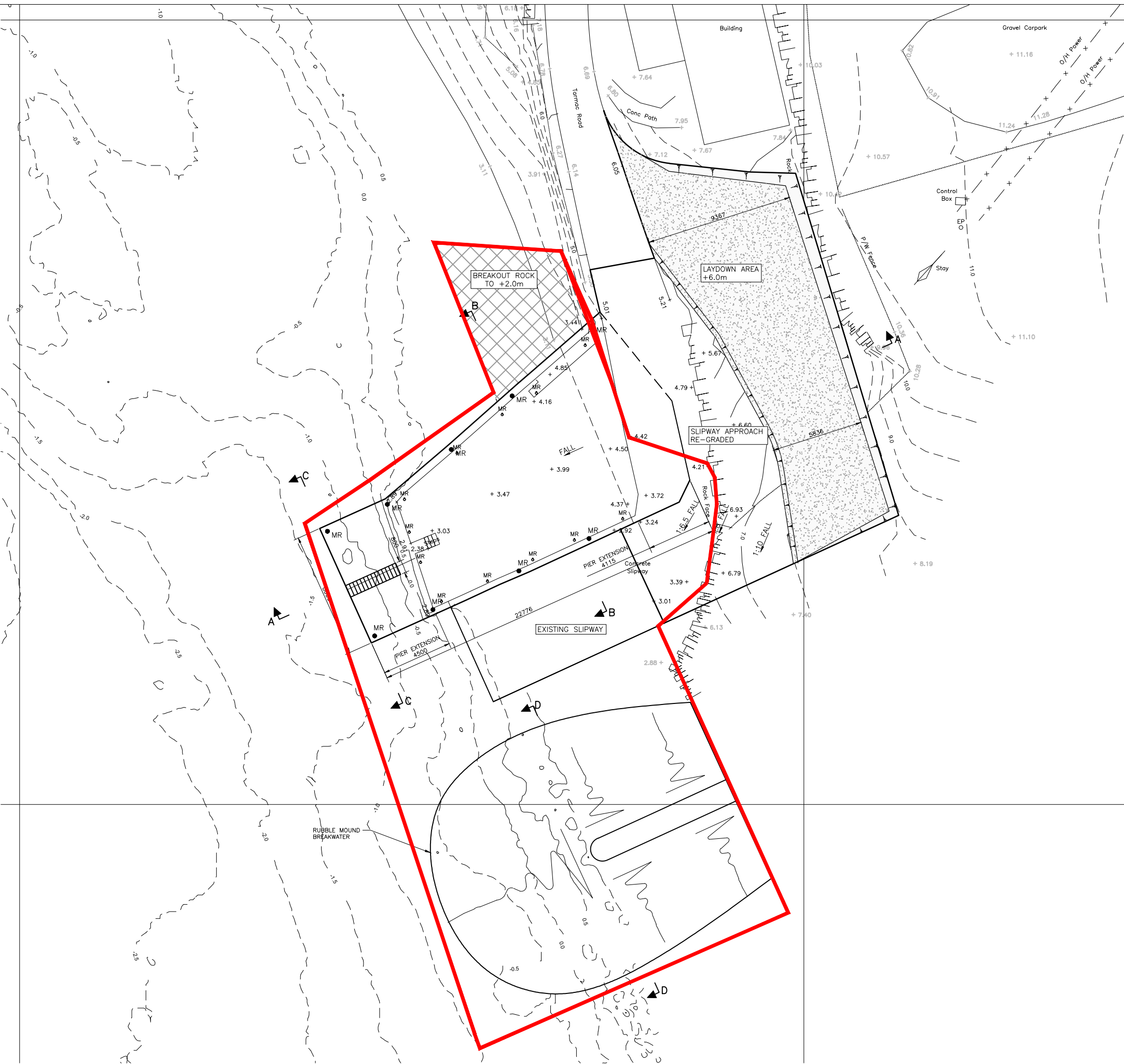
PLAN ON FERRY PIER SCALE 1:125
