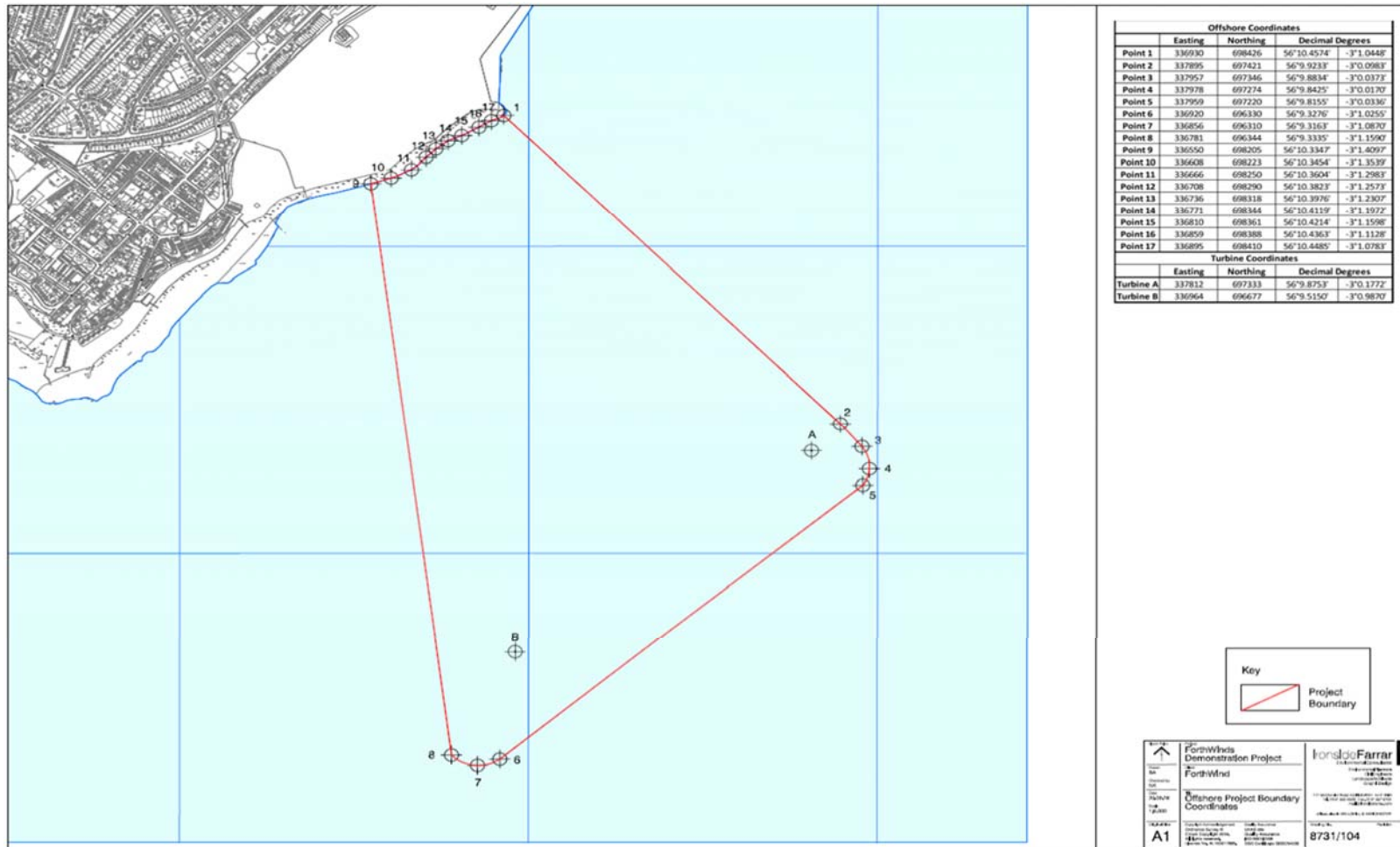
Figure 1 Fortwind Offshore Wind Generation Project Location showing Offshore Project Boundary and Phase 1 turbine deployment locations.
