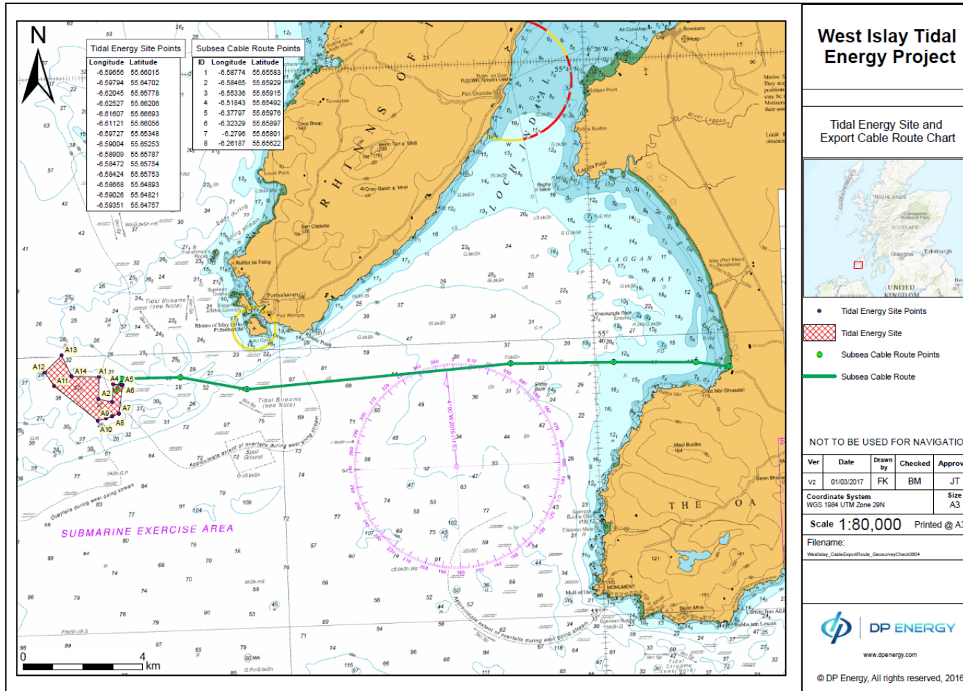
DP Marine Energy West Islay Tidal Energy Park location showing the Offshore Project Boundary and Export Cable Corridor to Kintra, Islay
